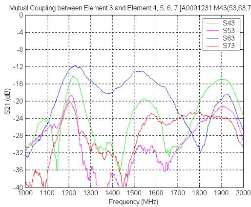
Figure 20 Mutual coupling between Element 3 and Element 4, 5, 6, and 7
