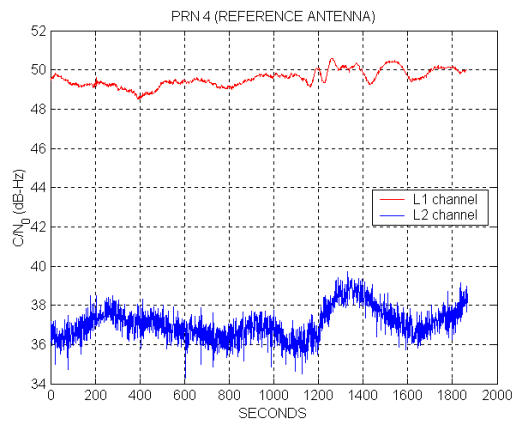
Figure 25 Measured C/N_0 of PRN 4 with a reference antenna (AT2775-16 from AeroAntenna Technology, Inc.)
