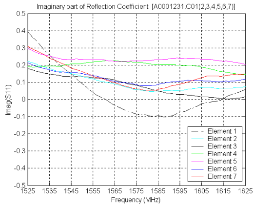
Figure 8 Imaginary part of the reflection coefficient of the seven antenna elements in the frequency band from 1525 to 1625 MHz
