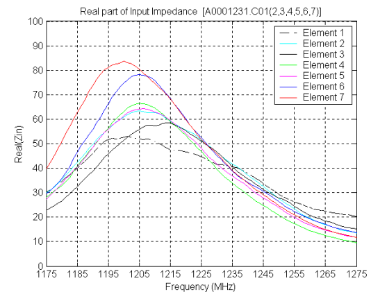
Figure 13 Real part of the input impedance of the seven antenna elements in the frequency band from 1175 to 1275 MHz
