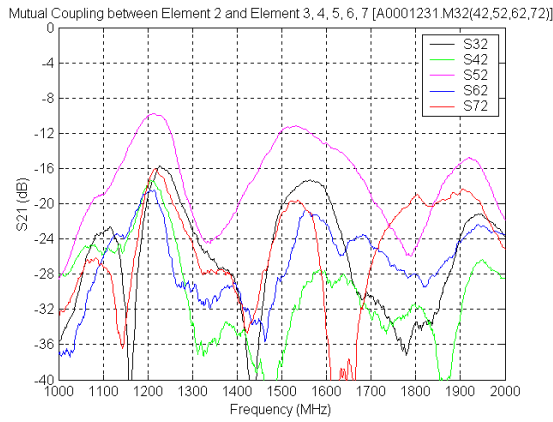
Figure 19 Mutual coupling between Element 2 and Element 3, 4, 5, 6, and 7
