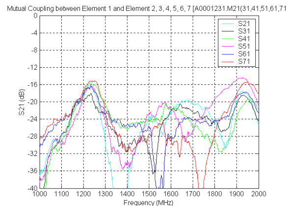
Figure 18 Mutual coupling between Element 1 (center element) and Element 2, 3, 4, 5, 6, and 7
