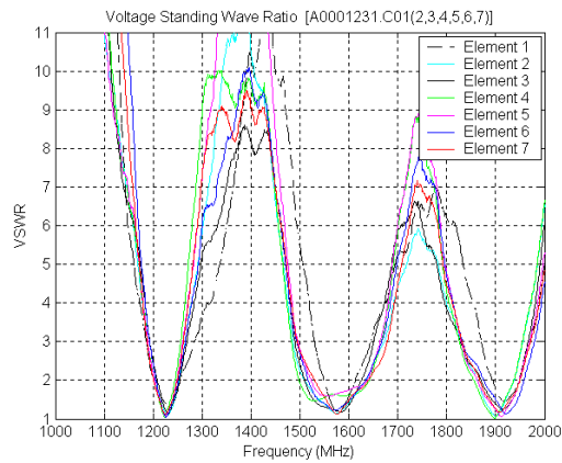
Figure 9 Voltage standing wave ratio of the seven antenna elements in the frequency band from 1000 to 2000 MHz
