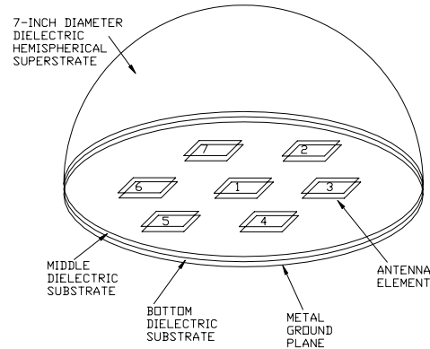
Figure 2 Configuration and dimensions of NAVSYS' seven-inch seven-element dual-frequency (L1/L2) S-CRPA
