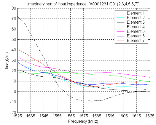
Figure 17 Imaginary part of the input impedance of the seven antenna elements in the frequency band from 1525 to 1625 MHz
