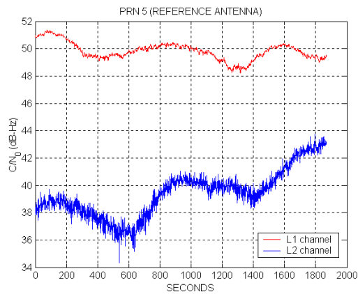
Figure 31 Measured C/N_0 of PRN 5 with a reference antenna (AT2775-16 from AeroAntenna Technology, Inc.)
