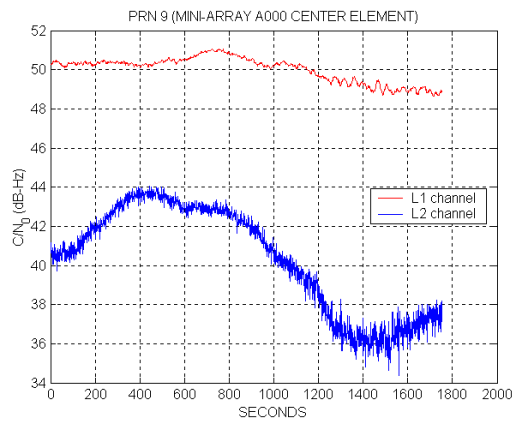
Figure 26 Measured C/N_0 of PRN 9 with Element 1 of S-CRPA
