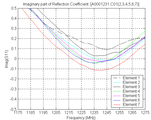
Figure 7 Imaginary part of the reflection coefficient of the seven antenna elements in the frequency band from 1175 to 1275 MHz
