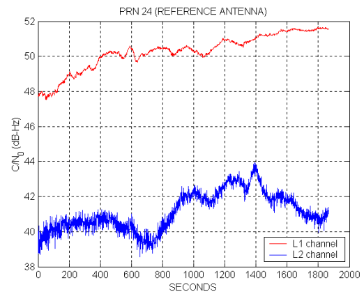
Figure 29 Measured C/N_0 of PRN 24 with a reference antenna (AT2775-16 from AeroAntenna Technology, Inc.)
