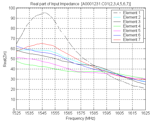
Figure 14 Real part of the input impedance of the seven antenna elements in the frequency band from 1525 to 1625 MHz
