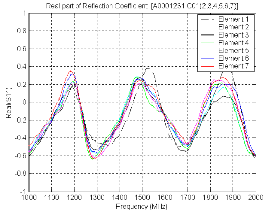
Figure 3 Real part of the reflection coefficient of the seven antenna elements in the frequency band from 1000 to 2000 MHz
