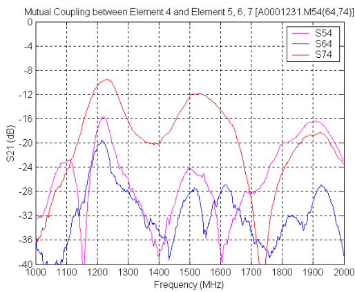
Figure 21 Mutual coupling between Element 4 and Element 5, 6, and 7
