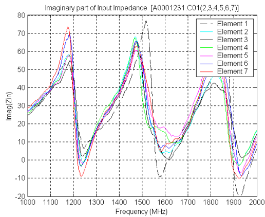
Figure 15 Imaginary part of the input impedance of the seven antenna elements in the frequency band from 1000 to 2000 MHz
