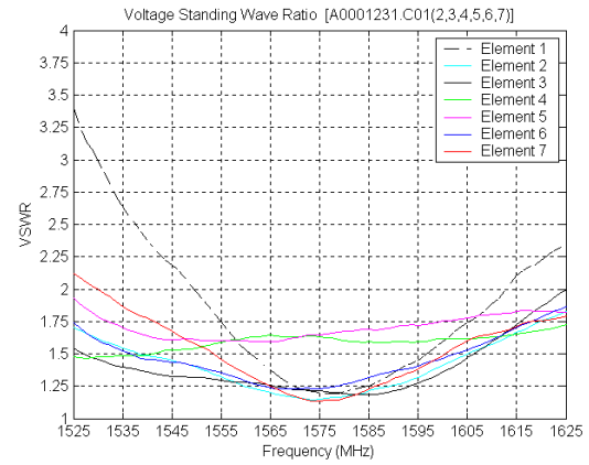
Figure 11 Voltage standing wave ratio of the seven antenna elements in the frequency band from 1525 to 1625 MHz
