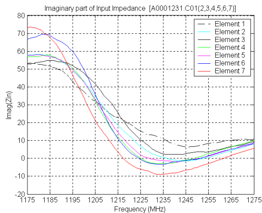
Figure 16 Imaginary part of the input impedance of the seven antenna elements in the frequency band from 1175 to 1275 MHz
