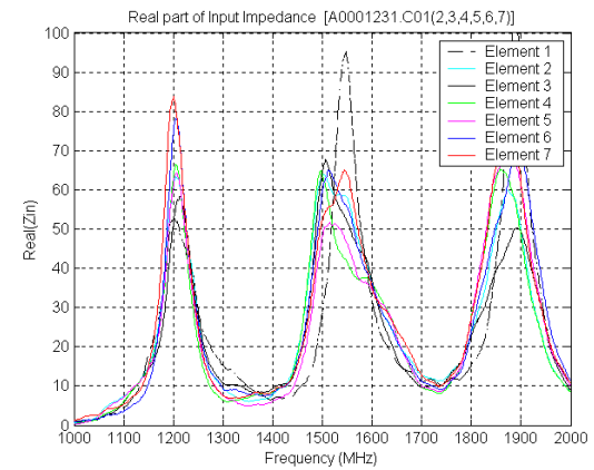
Figure 12 Real part of the input impedance of the seven antenna elements in the frequency band from 1000 to 2000 MHz
