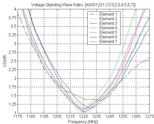
Figure 10 Voltage standing wave ratio of the seven antenna elements in the frequency band from 1175 to 1275 MHz
