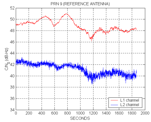
Figure 27 Measured C/N_0 of PRN 9 with a reference antenna (AT2775-16 from AeroAntenna Technology, Inc.)
