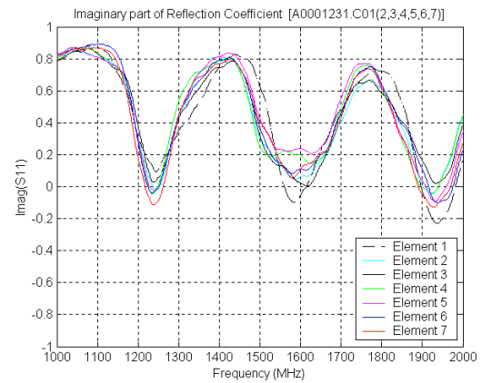
Figure 6 Imaginary part of the reflection coefficient of the seven antenna elements in the frequency band from 1000 to 2000 MHz
