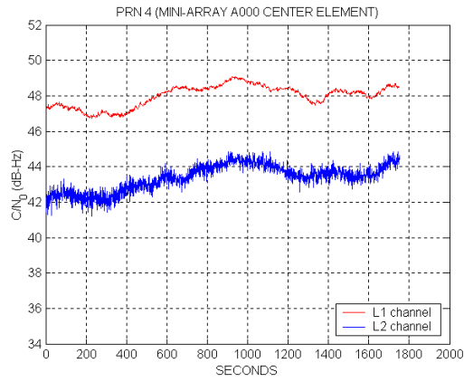
Figure 24 Measured C/N_0 of PRN 4 with Element 1 of S-CRPA
