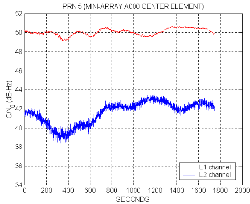
Figure 30 Measured C/N_0 of PRN 5 with Element 1 of S-CRPA
