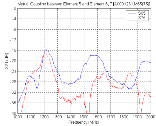
Figure 22 Mutual coupling between Element 5 and Element 6 and 7
