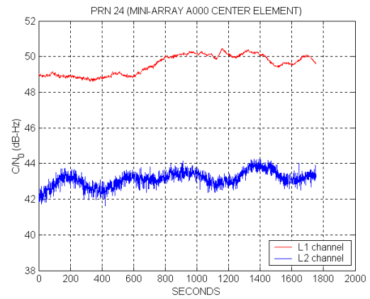
Figure 28 Measured C/N_0 of PRN 24 with Element 1 of S-CRPA
