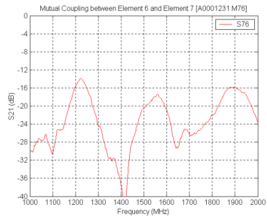
Figure 23 Mutual coupling between Element 6 and Element 7
