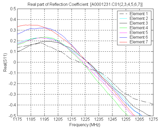
Figure 4 Real part of the reflection coefficient of the seven antenna elements in the frequency band from 1175 to 1275 MHz
