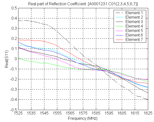
Figure 5 Real part of the reflection coefficient of the seven antenna elements in the frequency band from 1525 to 1625 MHz
