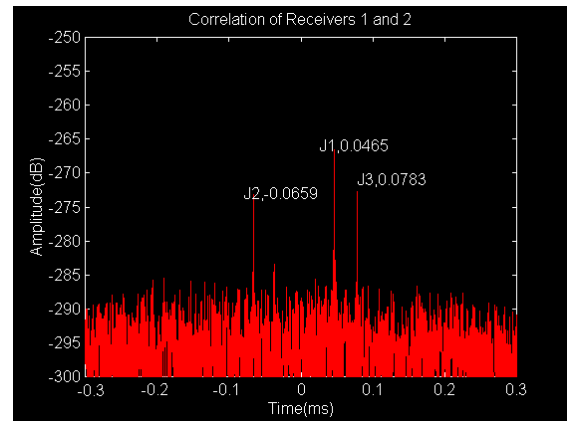
Figure 18 TDOA Jammer Simulated Data Results
