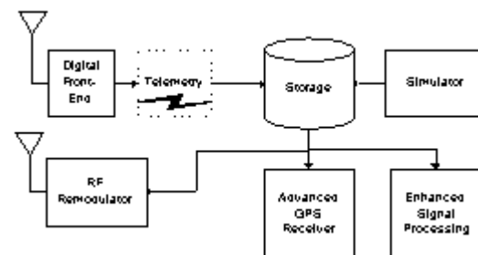
Figure 1 Digital Storage Receiver Architecture
