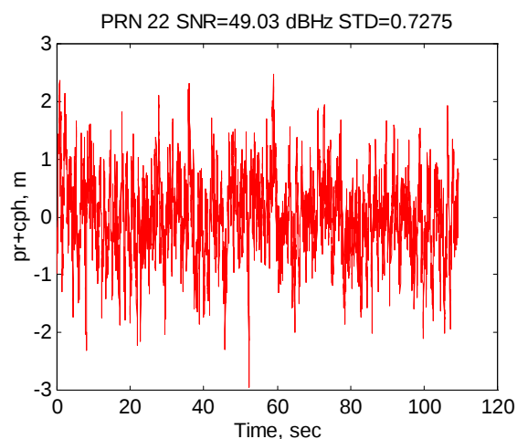
Figure 19 HAGR Difference between Pseudo-Range and Carrier Phase for PRN 22
