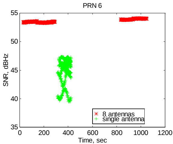
Figure 6 Signal Noise Ratio Comparison between Single Antenna and 8 Antennas for PRN 6
