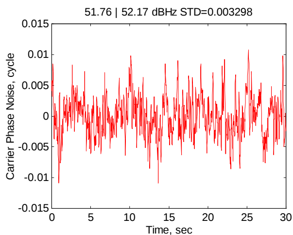
Figure 30 Single Differenced HAGR Carrier Phase Noise between PRN 30 and PRN 15
