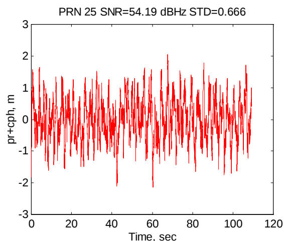
Figure 20 HAGR Difference between Pseudo-Range and Carrier Phase for PRN 25
