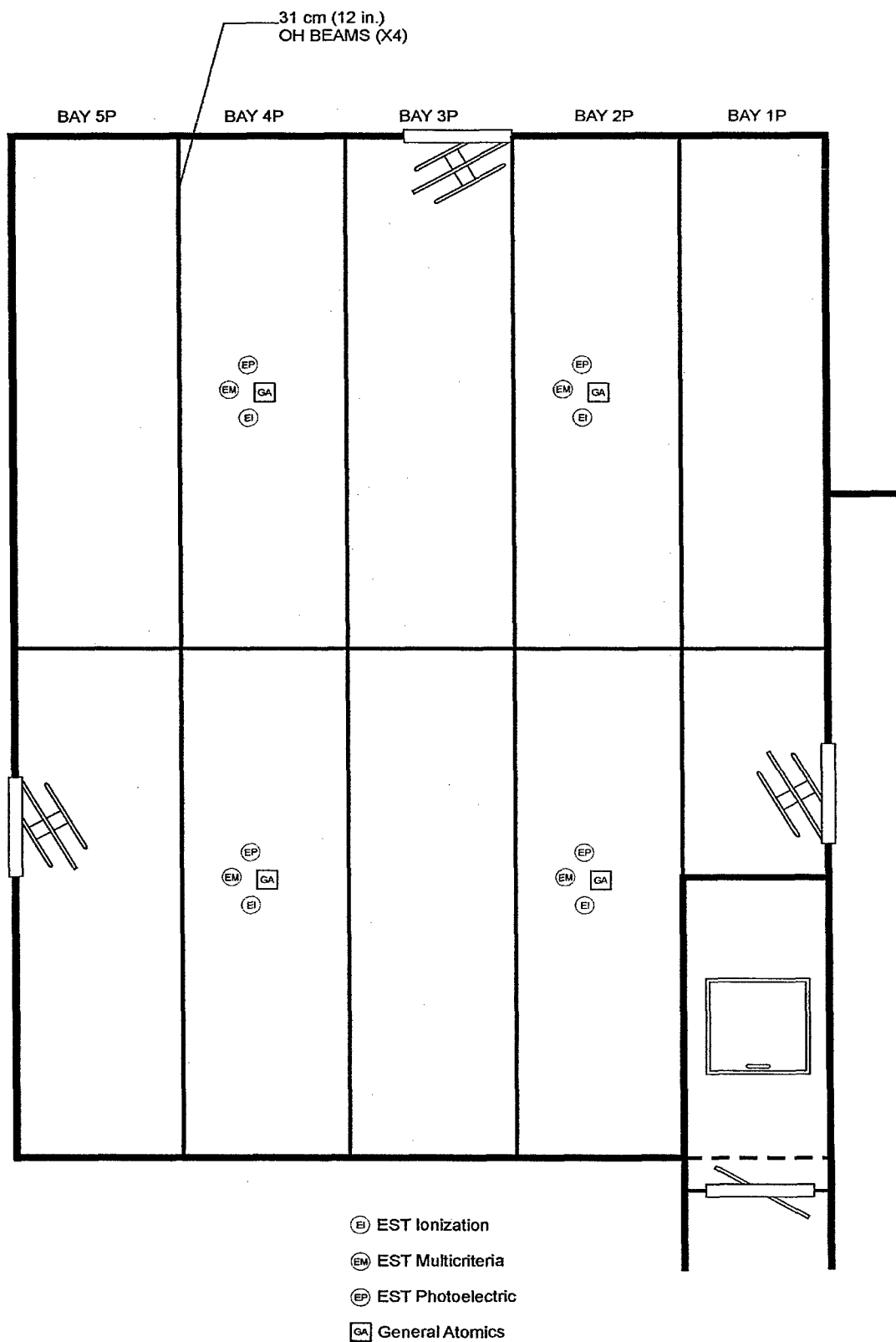
Fig. 12 — Locations of spot-type detectors in test compartment
