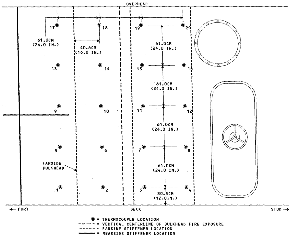
Fig. 11 — Locations of forward bulkhead thermocouples
