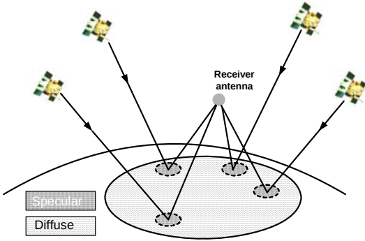
Figure 1 GPS Bistatic Geometry with Specular Reflection Points
