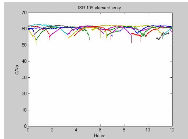
Figure 26 C/No values from the 109 element array
