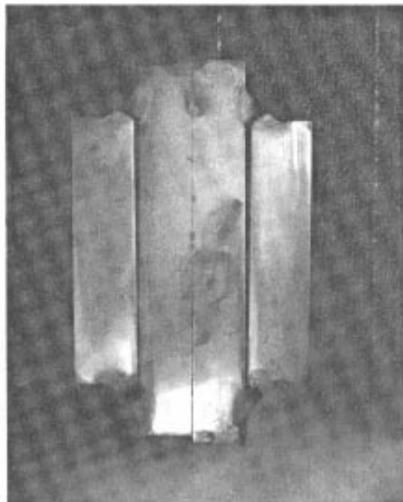
Figure 9. Longitudinal Shear Test Specimen 1A
