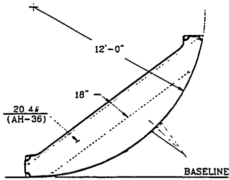
FIGURE 4 BILGE BRACKET
