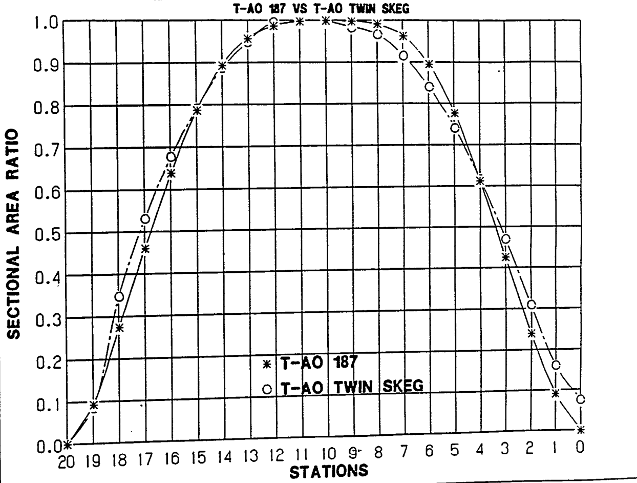
FIGURE 2 COMPARISON OF SECTIONAL AREAS
