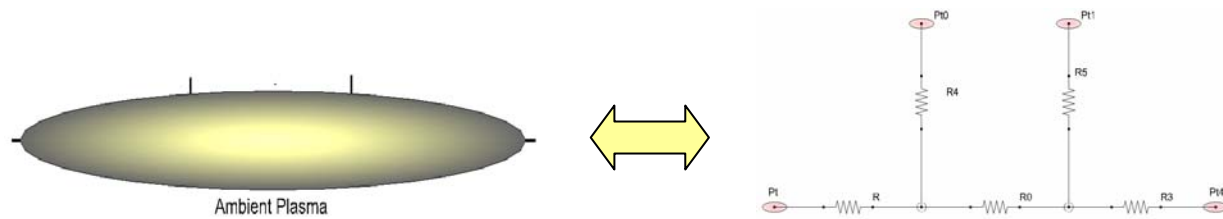
Figure 12. VTB Model for ambient plasma
