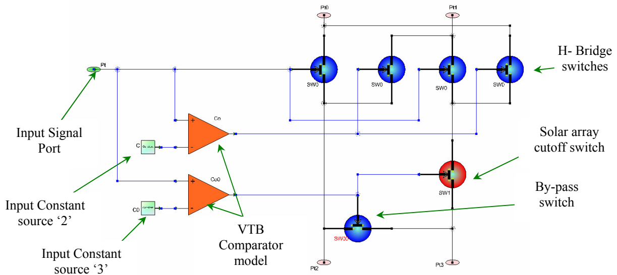
Figure 11. Schematic of the high voltage power switching module
