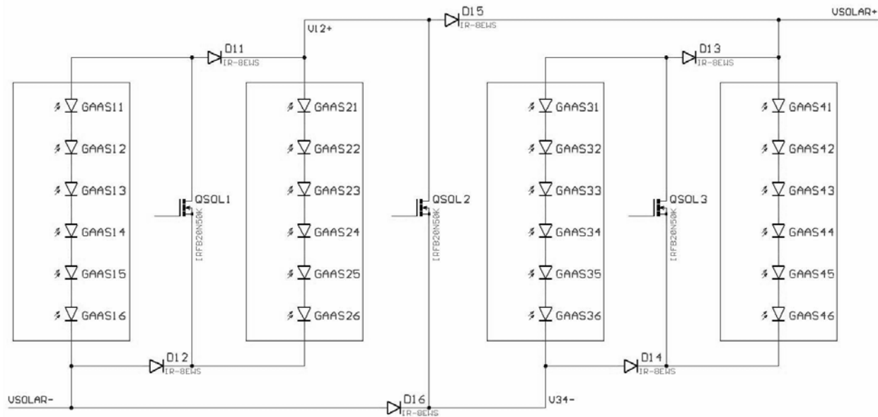
Figure 4. Series/parallel switching of 4 solar array strings
