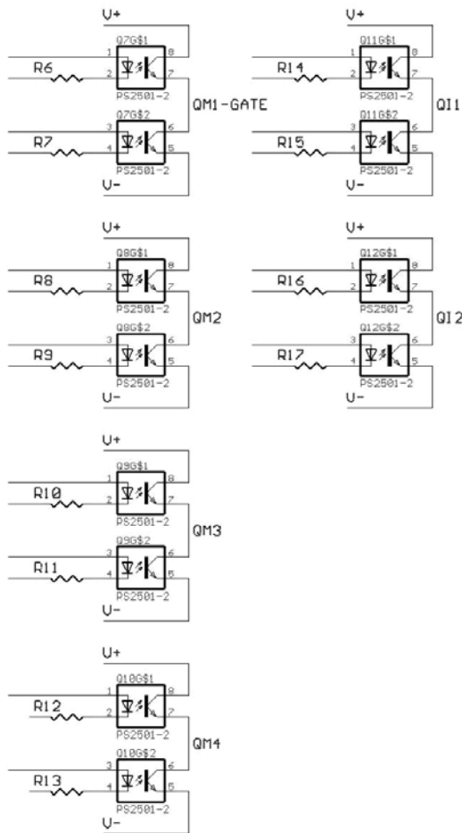
Figure 3. Opto-Isolated gate drive circuits, and H-bridge with IGBT-controlled shunts
