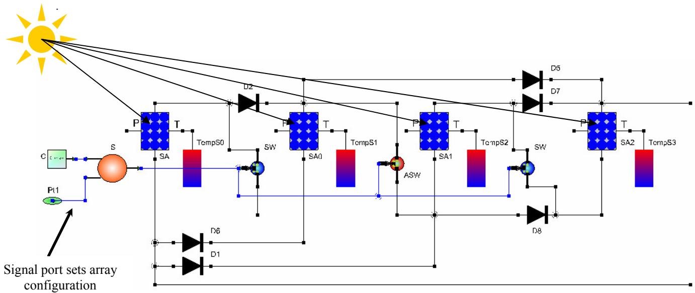
Figure 9. Internal Schematic diagram of solar array power module
