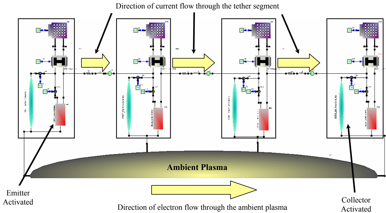
Figure 7. Controlling the direction of current in the tether with switching control
