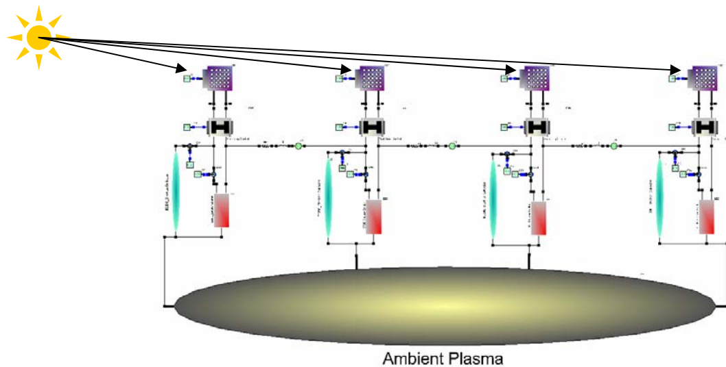
Figure 5. VTB schematic, showing the EDDE configuration
