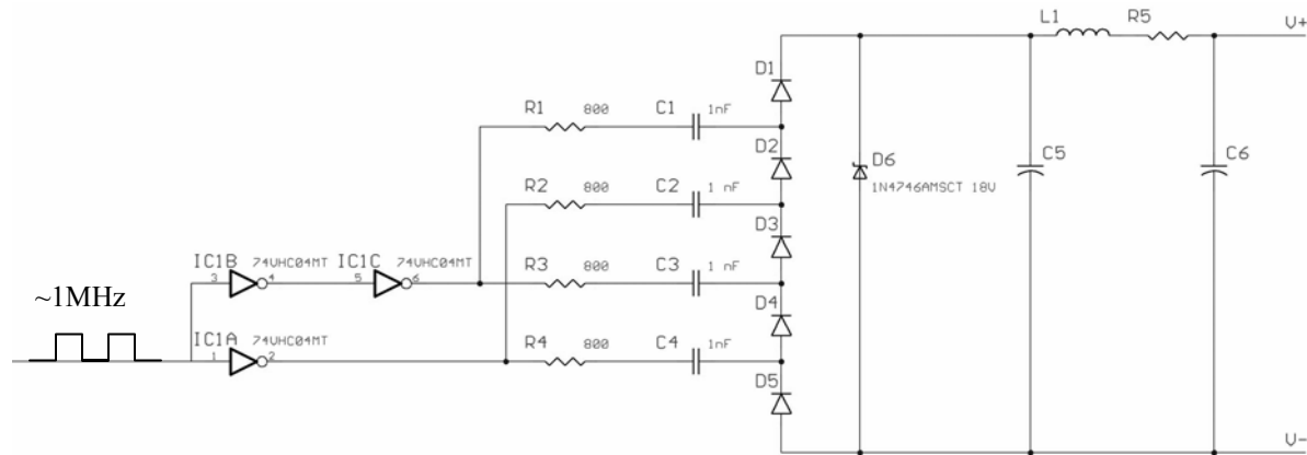
Figure 2. DC-isolated charge-pump for MOSFET and IGBT gate drive (one of 8)
