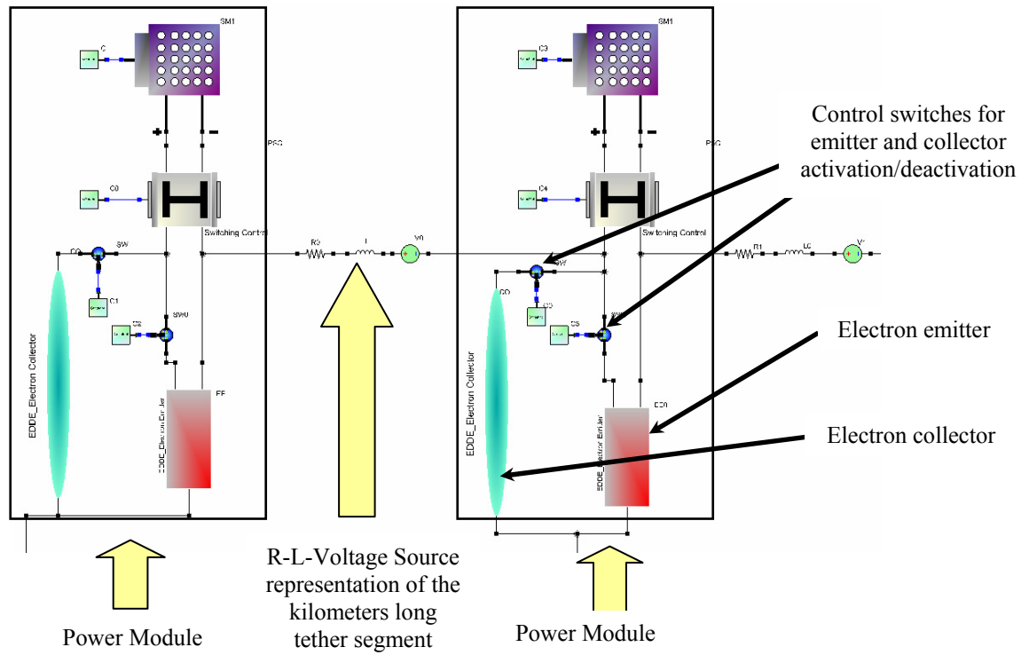
Figure 6. Configuration of single tether segment in VTB
