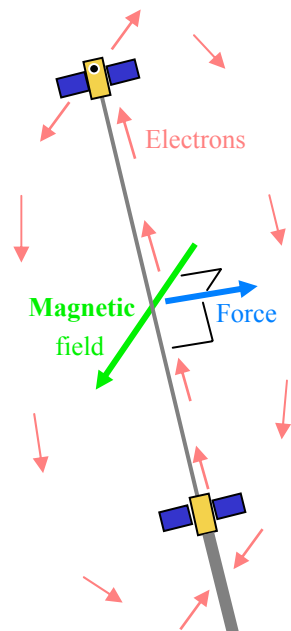
Figure 1. Electrodynamic loop and force
