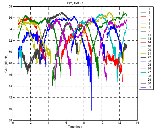
Figure 7 P(Y) HAGR Signal-to-Noise (dB-Hz)
