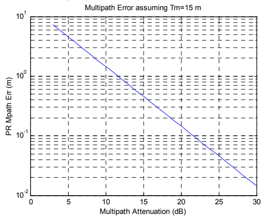
Figure 17 Peak Multipath Pseudo-Range Error
