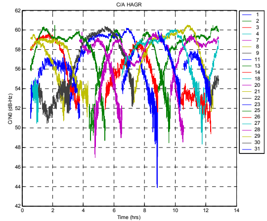
Figure 6 C/A HAGR Signal-to-Noise (dB-Hz)
