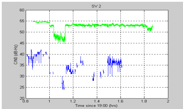
Figure 26 SV 2 C/N0
