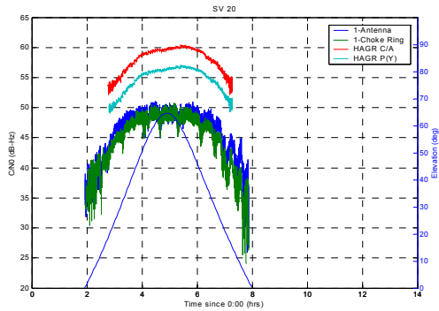
Figure 21 Signal/Noise Ratio SV 20
