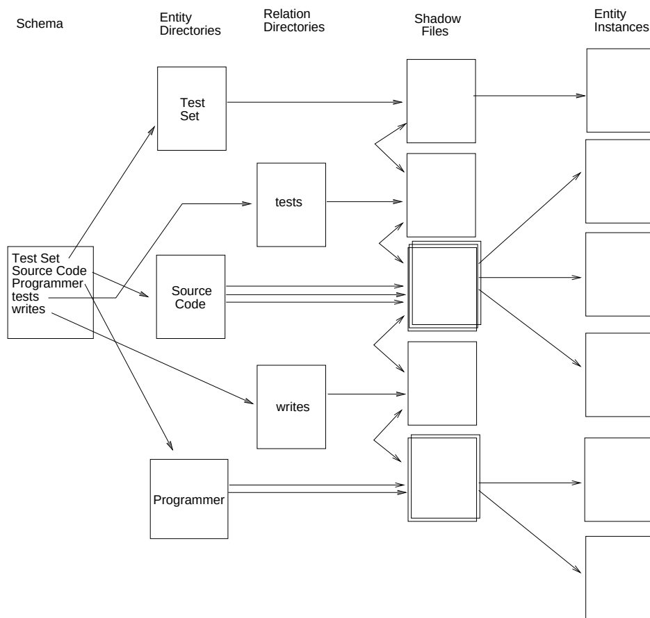
Figure 4: An Example of Labyrinth's Logical Structure.
