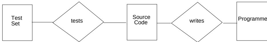
Figure 2: A Simple Entity-Relationship (E-R) Diagram.
