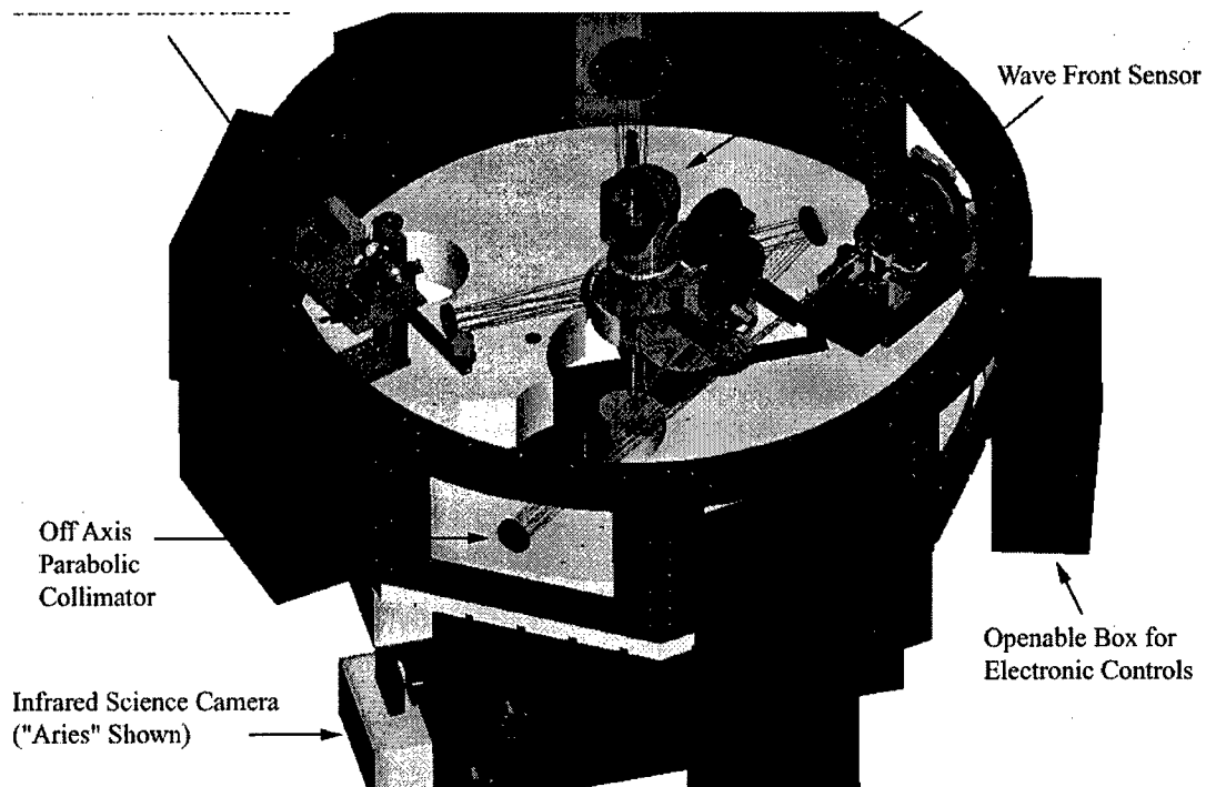
Fig. 3. Wavefront sensor "Top Box" from the MMT AO system.
