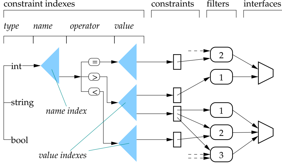
Figure 6: Generic Four-Level Representation of the Forwarding Table
