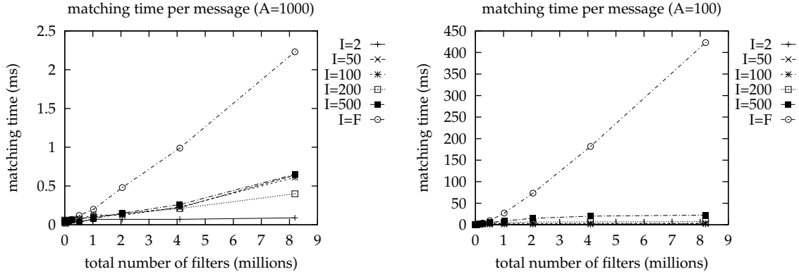
Figure 9: Overall Performance of the Forwarding Algorithm
