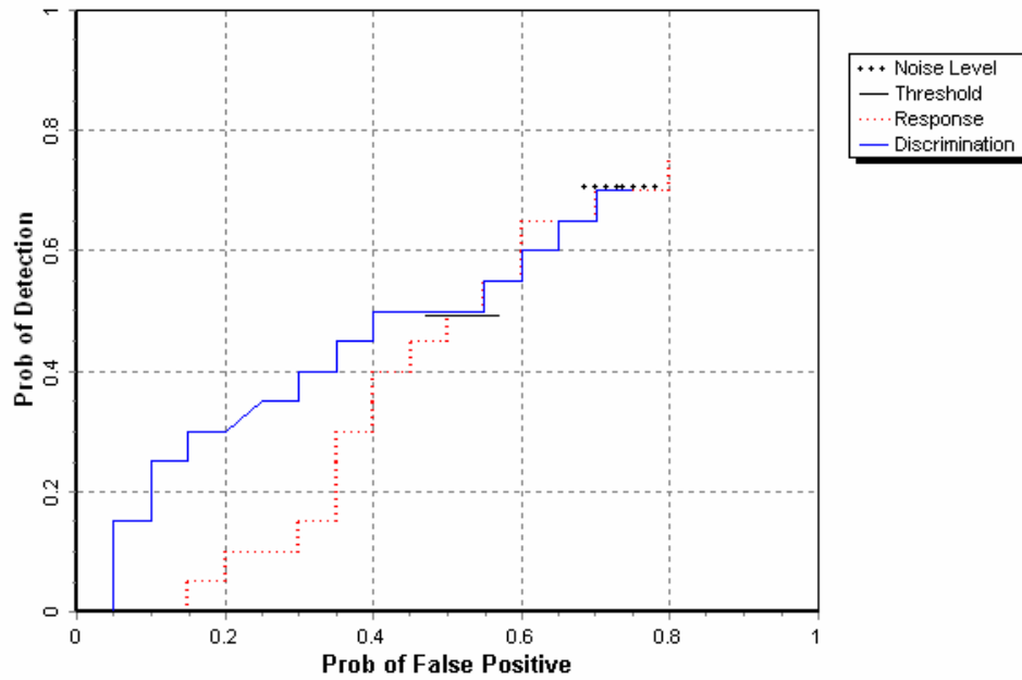
Figure 4. GEM-5/man-portable blind grid probability of detection for response and discrimination stages versus their respective probability of false positive for all ordnance larger than 20 mm.
