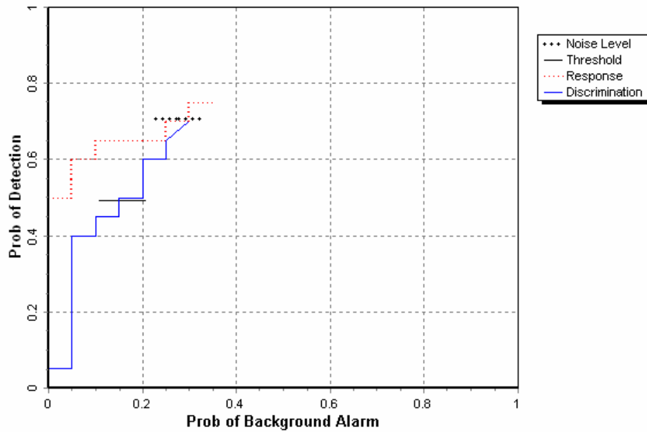
Figure 5. GEM-5/man-portable blind grid probability of detection for response and discrimination stages versus their respective probabilities of background alarm for all ordnance larger than 20 mm.
