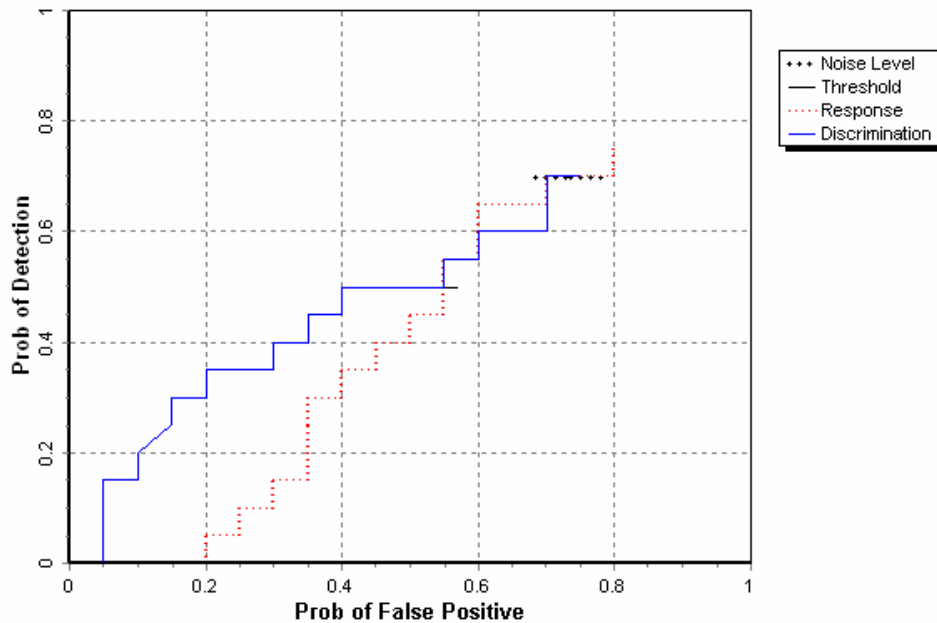
Figure 2. GEM-5/man-portable blind grid probability of detection for response and discrimination stages versus their respective probability of false positive over all ordnance categories combined.
