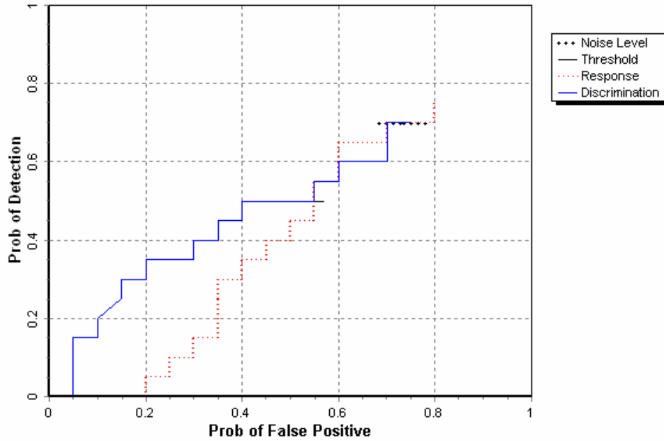
Figure 3. GEM-5/man-portable blind grid probability of detection for response and discrimination stages versus their respective probability of background alarm over all ordnance categories combined.
