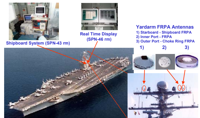
Figure 4 Shipboard Relative GPS Carrier Landing Test Installation
