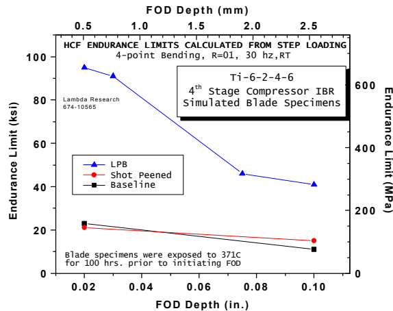
Figure 11: Effect of FOD size on the fatigue strength ( 10^7 cycle endurance limit) of blade-edge specimens.
