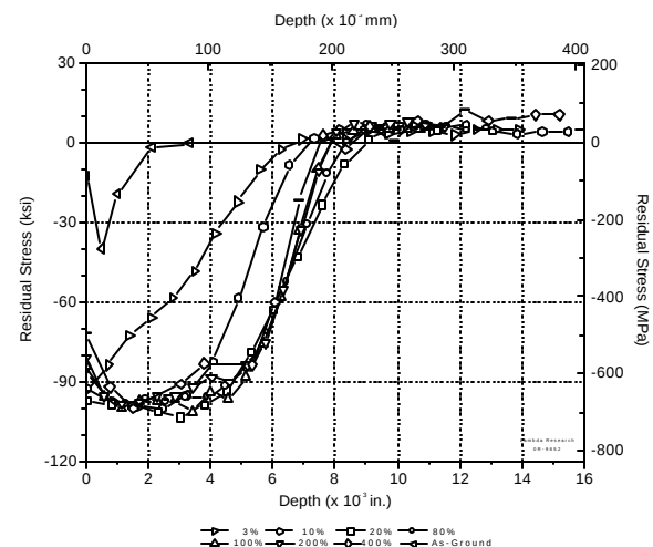
Figure 2. Residual stress-depth distributions for various coverage levels. Coverage is defined as the ratio of time to produce 100% surface impacts.
