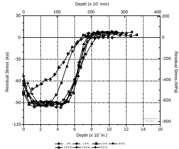
Figure 4. Residual stress-depth distributions after thermal exposure (475F/24 hr.)
