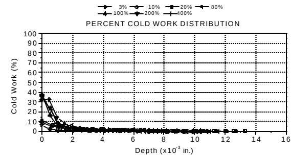
Figure 5. Cold work-depth distributions after thermal exposure (475F/24 hr.)
