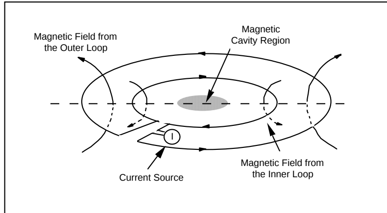
Figure 2. Conceptual representation of the GEM-3 coils.
