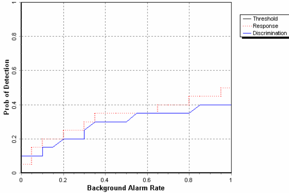
Figure 3. GEM-3 Realtime Disc/hand held mogul probability of detection for response and discrimination stages versus their respective background alarm rate over all ordnance categories combined.
