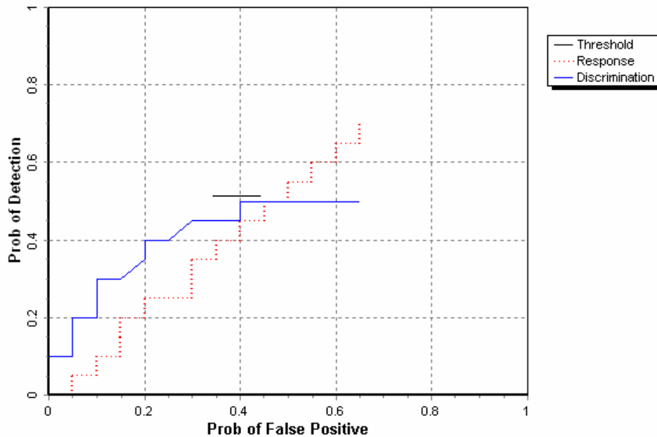
Figure 2. GEM-3 Realtime Disc/hand held mogul probability of detection for response and discrimination stages versus their respective probability of false positive over all ordnance categories combined.
