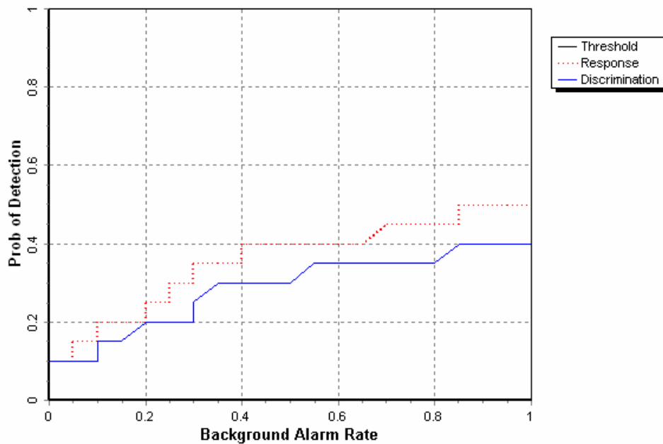
Figure 5. GEM-3 Realtime Disc/hand held mogul probability of detection for response and discrimination stages versus their respective background alarm rate for all ordnance larger than 20 mm.
