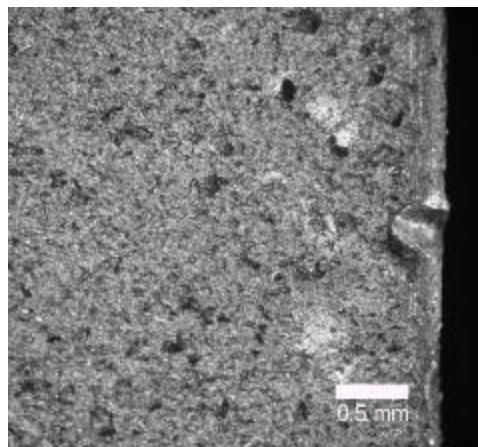
Figure 1 – Typical FOD showing a single large impact on the leading edge, concave side, of the Ti-6Al-4V first stage fan blade.
