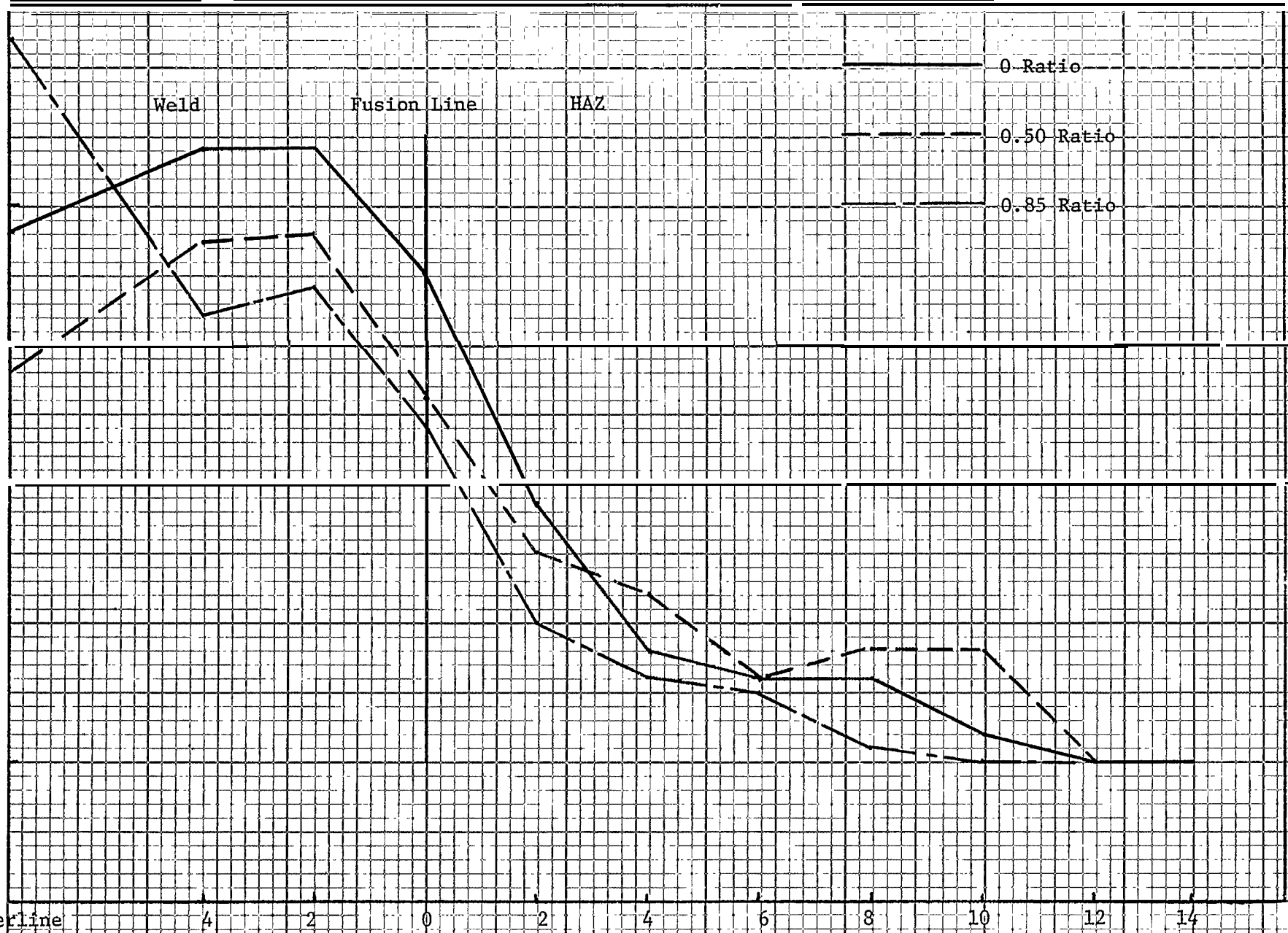
Figure 15. Hardness of Welds Produced With Hobart Fabco 81 Electrode
