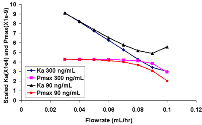
Figure 16: Simulated results for the k_a and P_{max} the baseline model generates given data from two site adsorption, one site flow dependent (80% of sites) and one site not (20%).
