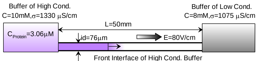
Figure 68: Schematic of the system used in coupled EOF/protein binding experiments and simulations
