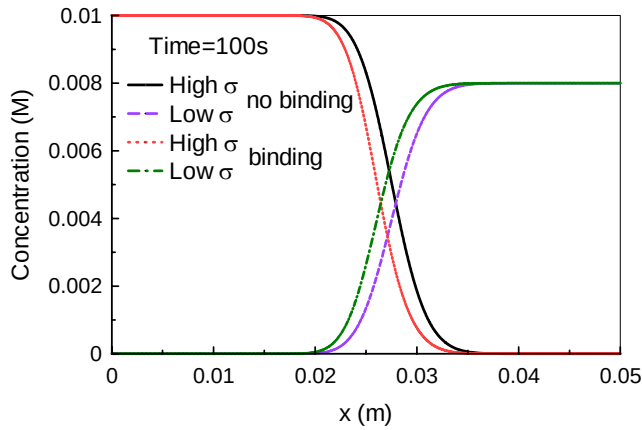
Figure 69: Comparison of buffer concentration at time t=100\text{s} for the cases of binding and no binding.
