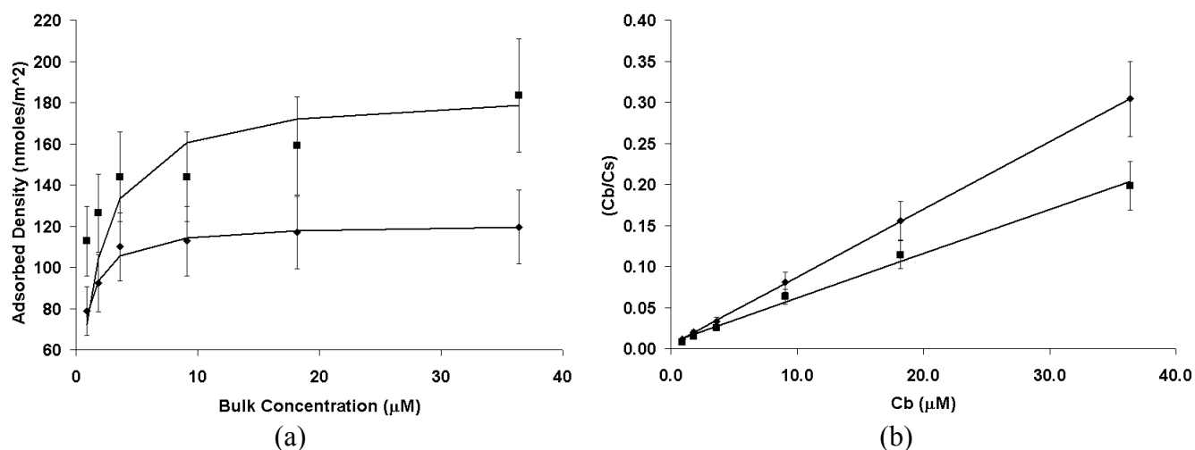
Figure 9: Static data for acid phosphatase (ACP). Diamonds represent data for PEEK and squares represent data for Teflon. Plots contain data as points with error bars and statistical fit shown as a solid curve. (a) Langmuir plot and (b) Lineweaver-Burke plot.
