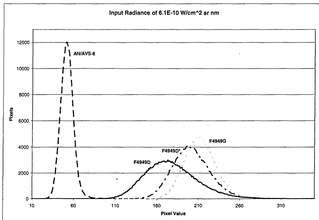
Figure 10. Noise histograms for four NVGs at the same input radiance of 6.1E-10 W/cm 2 sr nm.
