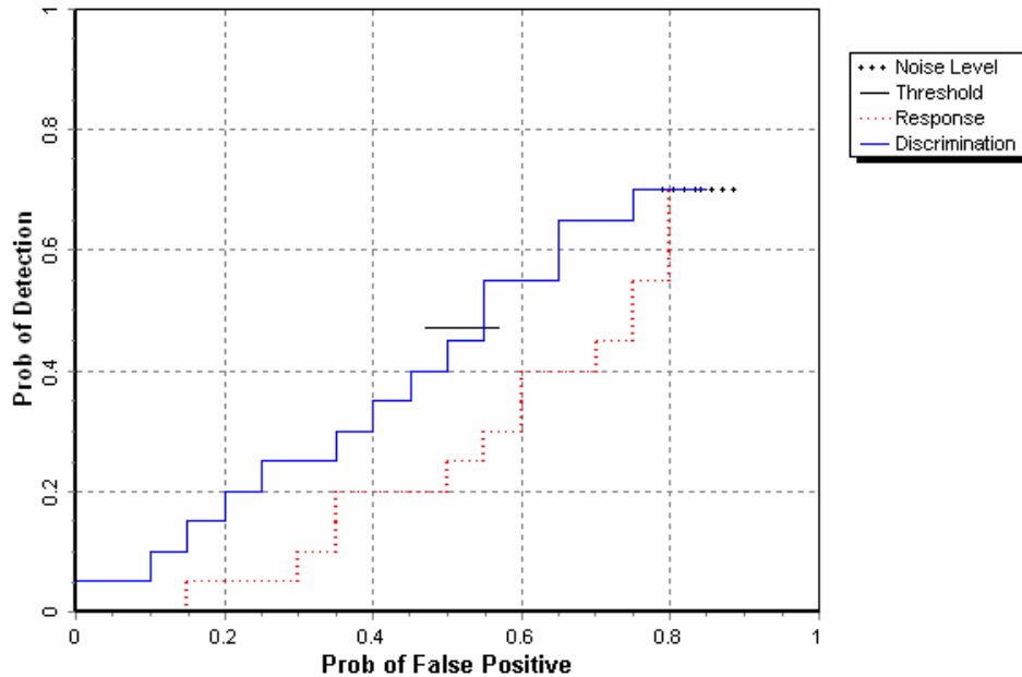
Figure 2. MTADS MAG/Towed Blind Grid probability of detection for response and discrimination stages versus their respective probability of false positive over all ordnance categories combined.
