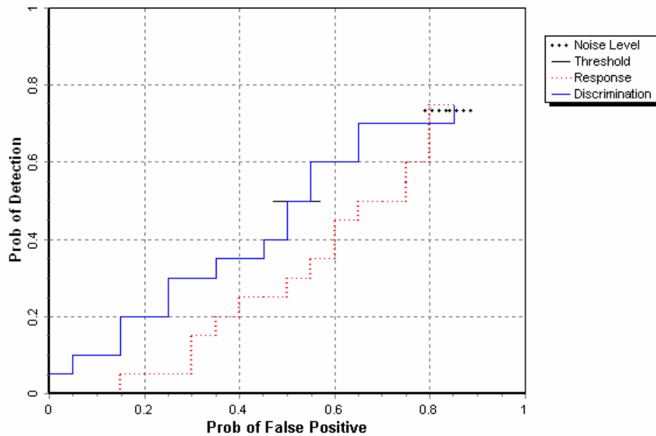
Figure 4. MTADS MAG/Towed Blind Grid probability of detection for response and discrimination stages versus their respective probability of false positive for all ordnance larger than 20 mm.
