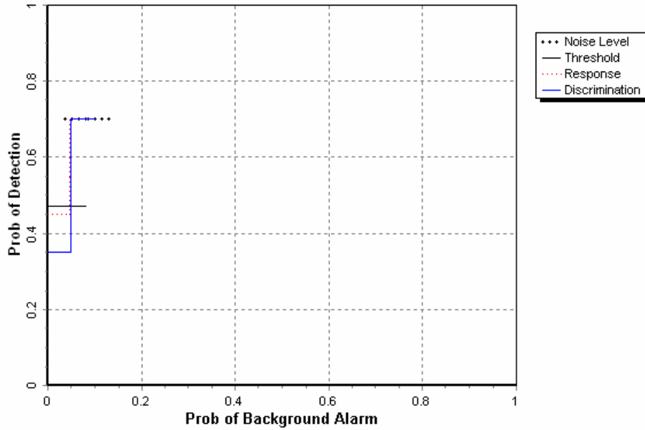
Figure 3. MTADS MAG/Towed Blind Grid probability of detection for response and discrimination stages versus their respective probability of background alarm over all ordnance categories combined.
