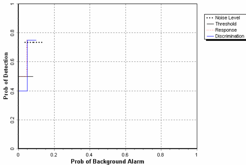
Figure 5. MTADS MAG/Towed Blind Grid probability of detection for response and discrimination stages versus their respective probability of background alarm for all ordnance larger than 20 mm.
