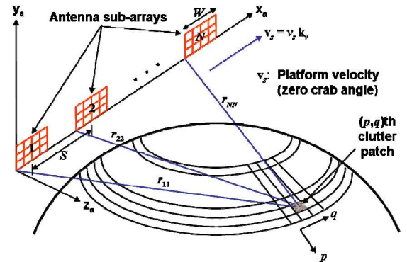
Figure 1. Scenario and platform formation for linear sparse array.
