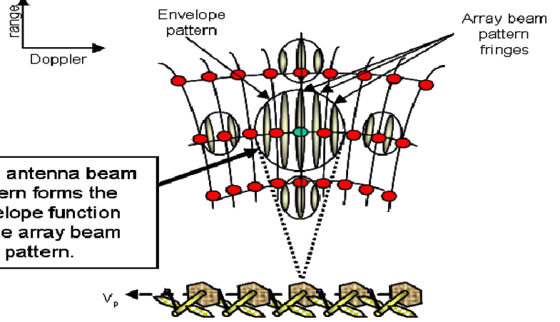
Figure 2. PRF sampling grid and antenna beam pattern.
