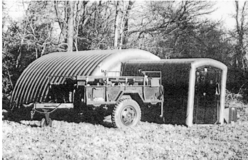
Figure 1. M-51 Collective Protection System.
