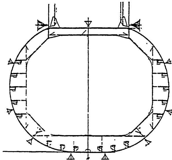
Figure 12. Lower Hull Structure Producibility Enhanced Design (PED)
