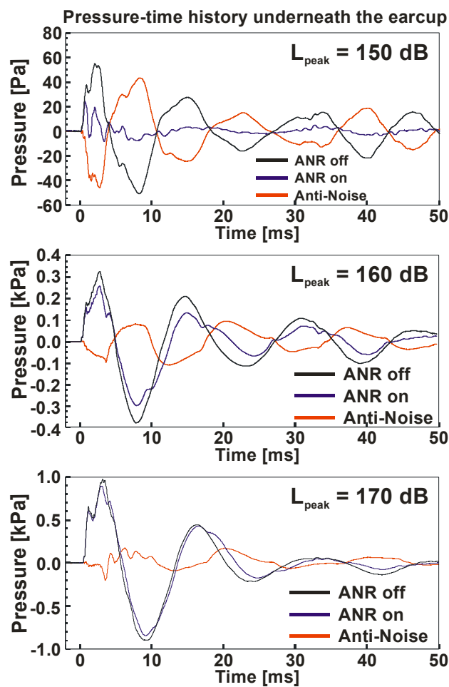
Figure 22: Pressure time histories underneath the hearing protector, when exposed to impulse noise.
