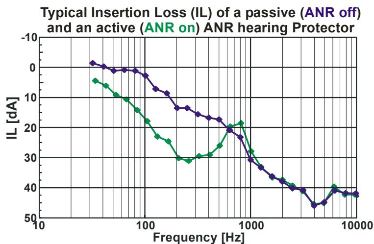
Figure 14: Insertion Loss (IL) for an ANR Hearing Protector wit ANR switches ON and OFF
