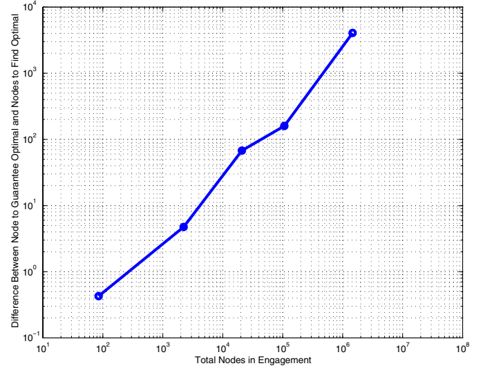
Fig. 2. Mean difference between number of nodes required to guarantee optimal and those required to find optimal assignments.
