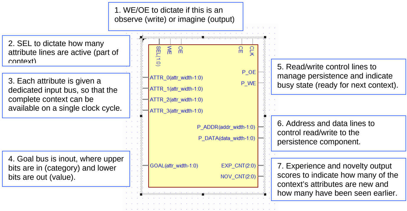
Figure 19: Symbol Schematic for Associative Memory Entity
