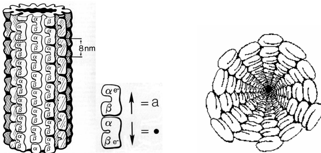
Figure 56: Microtubule with electron switching and electro-isolated interior
