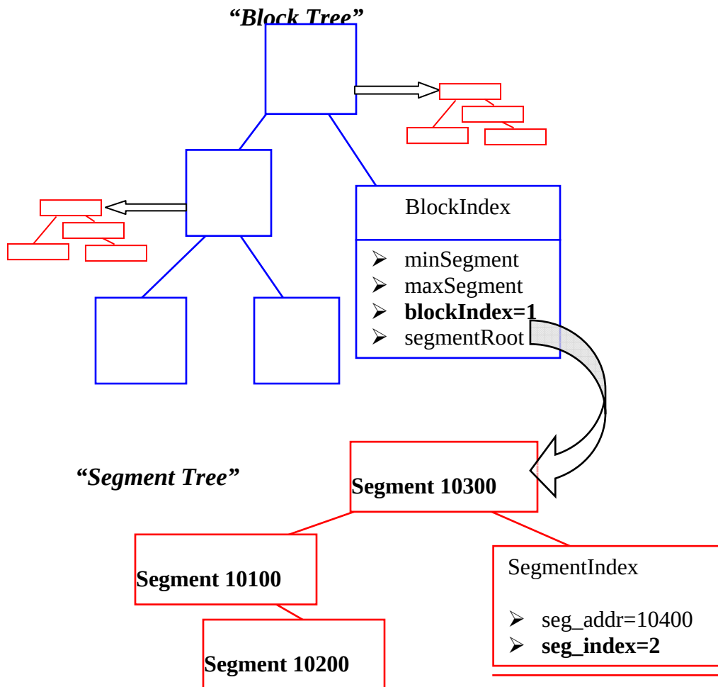
Figure 23: Indexing structures for blocks and segments
