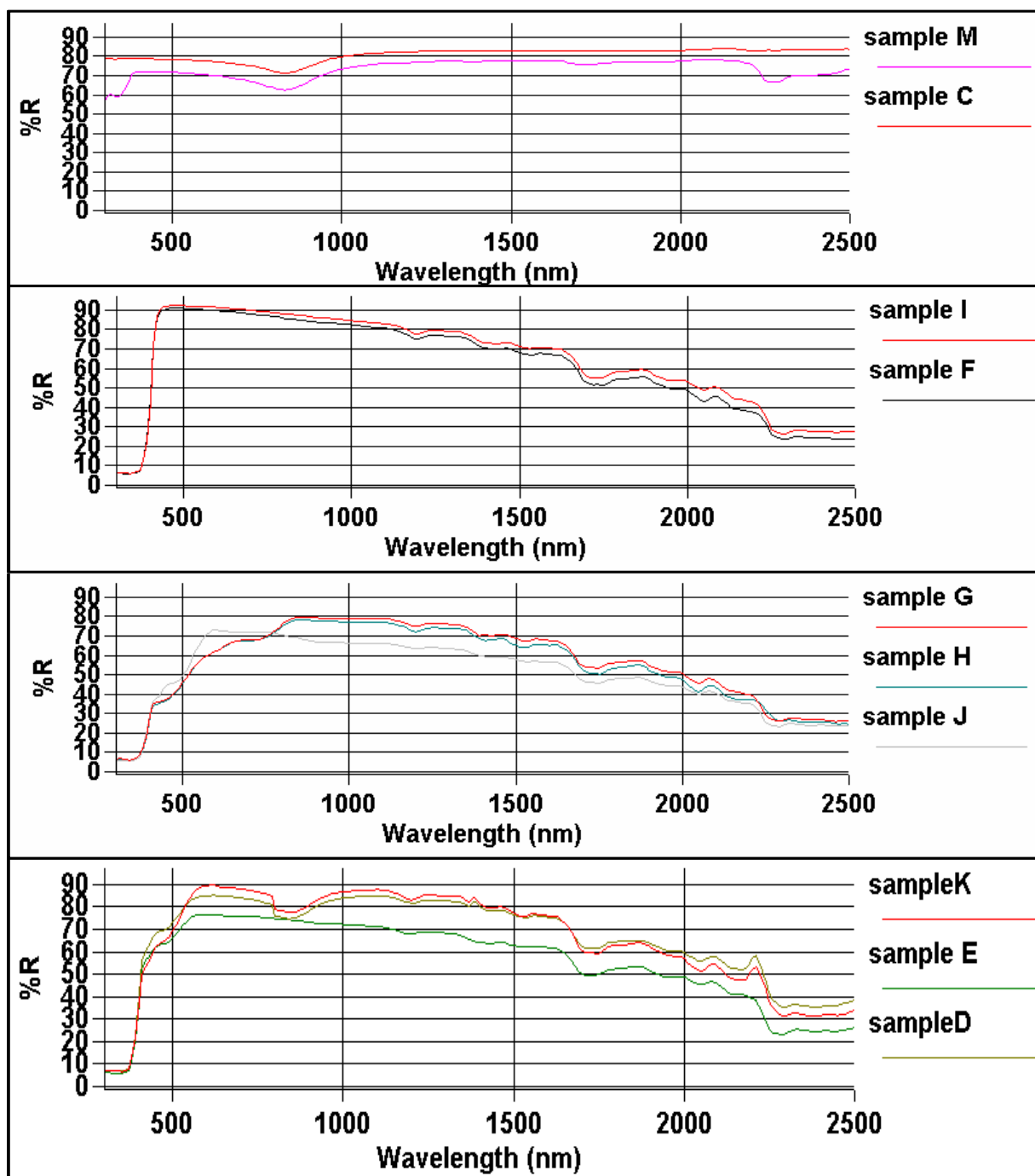
Figure 7. Reflectance properties of samples from the UV to NIR wavelengths.
