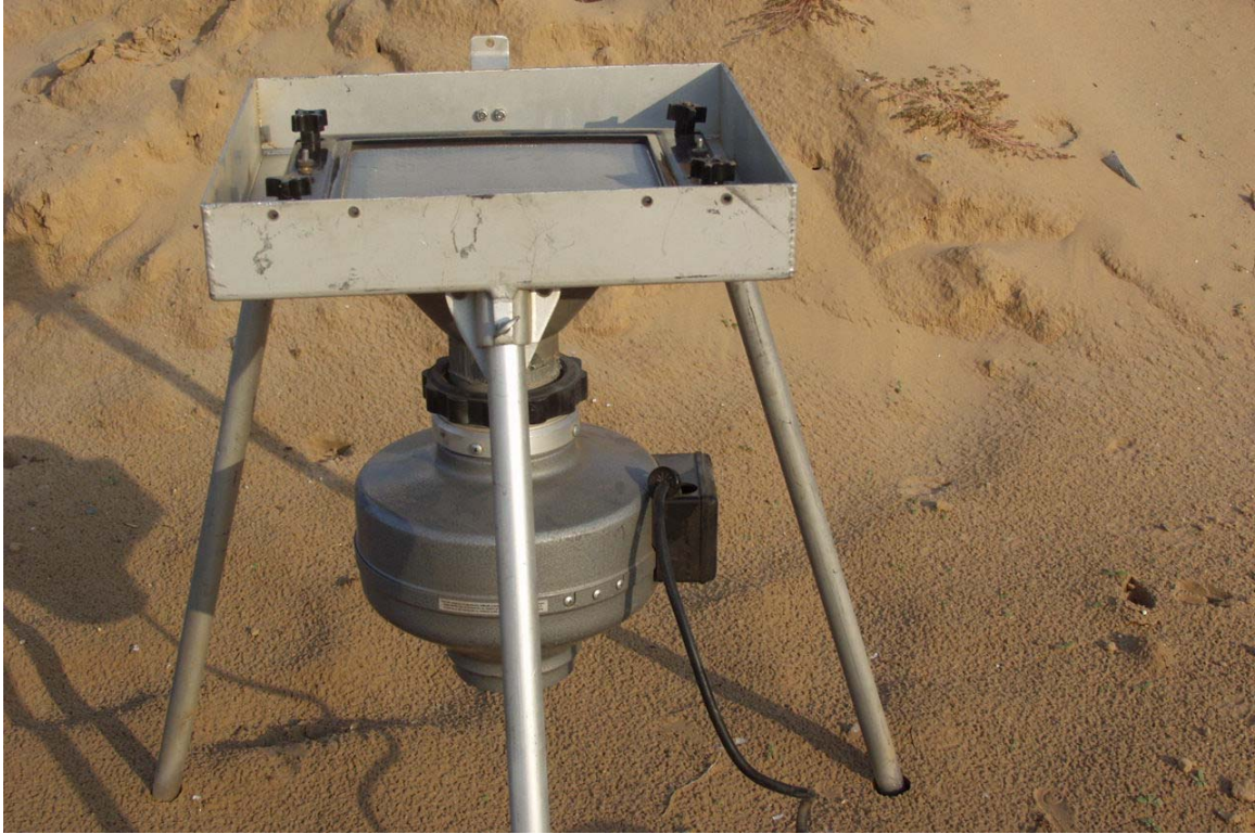
Photo 9. Dust collection system
