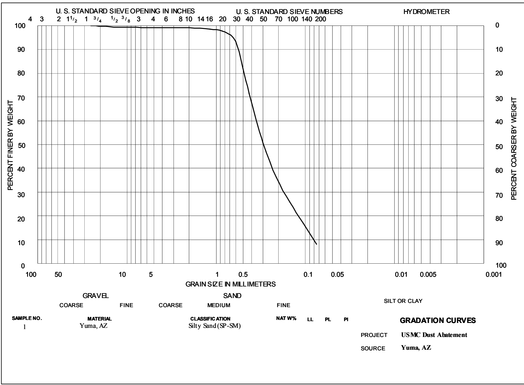
Figure 2. Grain size distribution for soil at testing location
