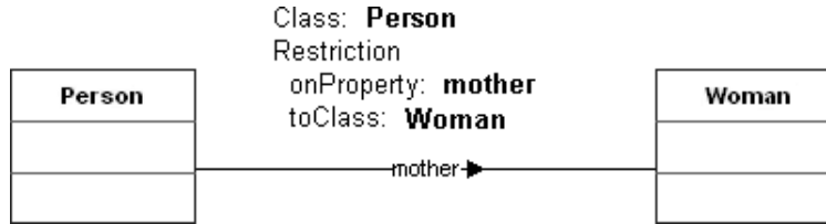
Fig. 2. DAML Property Restriction
