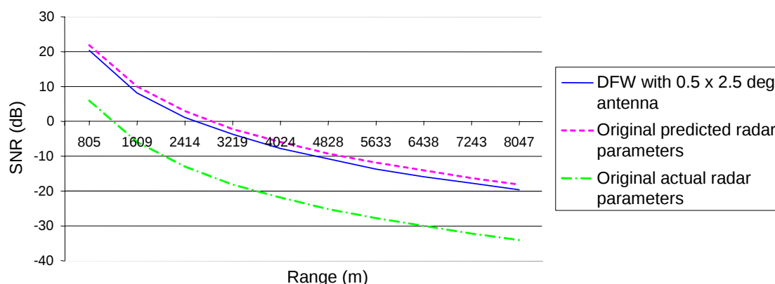
FIGURE 11-6. 94 GHZ BIRDAR TM SNR FOR ORIGINAL AND DFW AIRPORT RADAR CONFIGURATIONS ASSUMING BIRD FLOCK TARGETS WITH RCS = 0.03M 2 .
