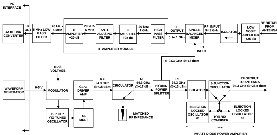
FIGURE 1-4. IMPATT TRANSCEIVER.
