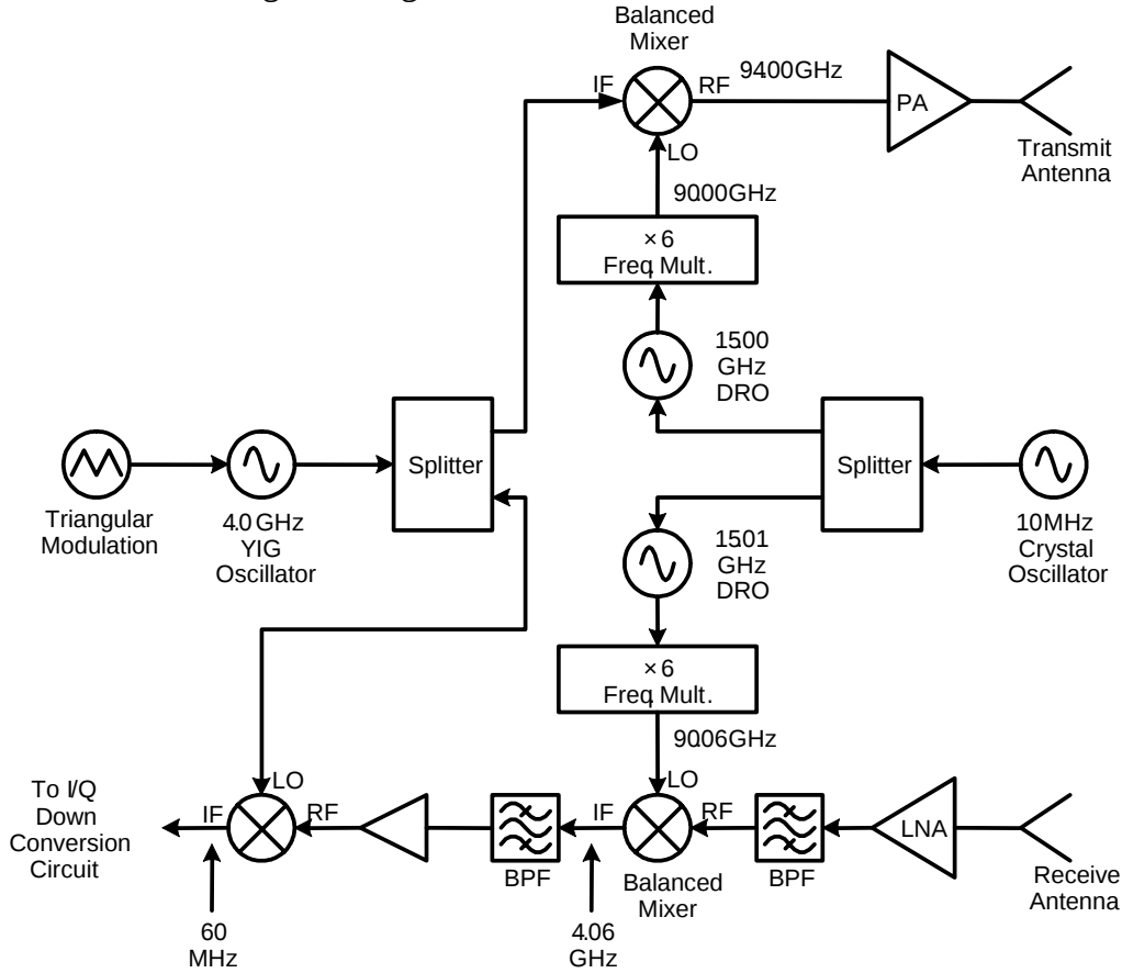
FIGURE 11-11. SUPERHETERODYNE TRANSCEIVER.
