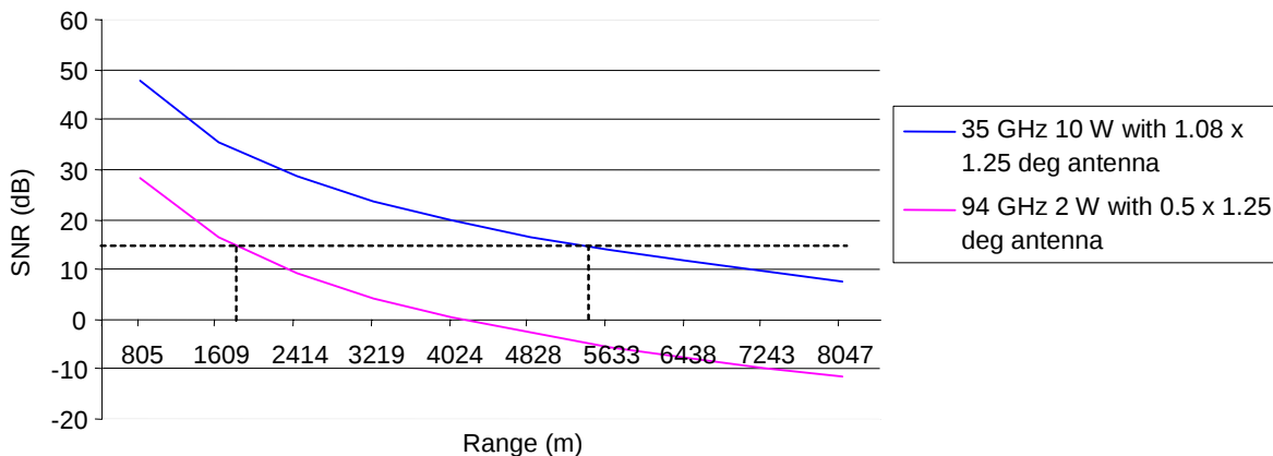
FIGURE 11-9. SNR FOR PROPOSED 35 AND 94 GHz BIRDAR™ RADARS ASSUMING BIRD FLOCK TARGETS WITH RCS = 0.03M 2 .
