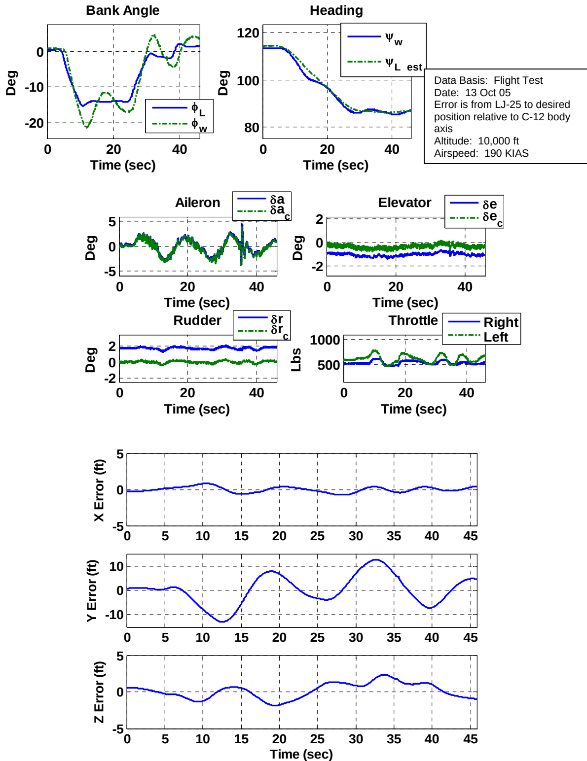
Figure 24. Maneuver 6:10. Precontact, 15 deg Bank Turn.
