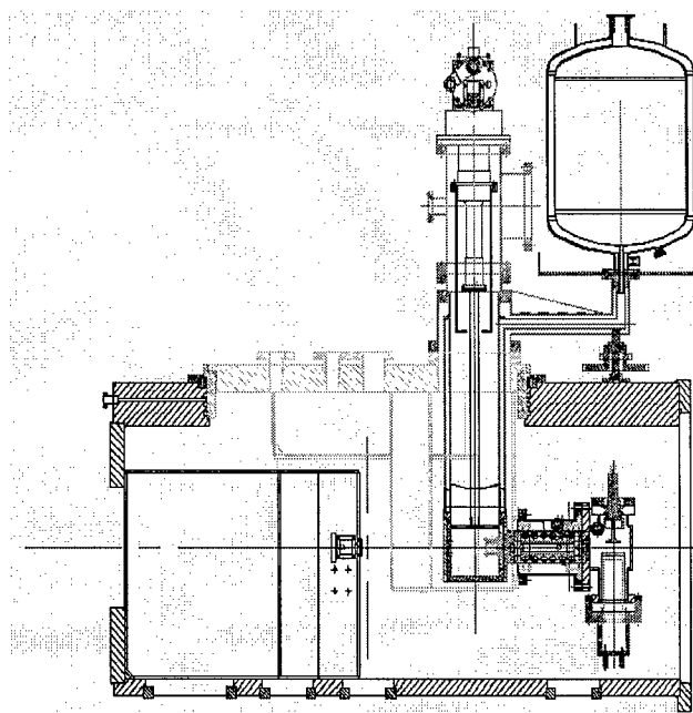
Figure 1: (Top) Top view of the experimental setup with differentially pumped regions I – III, source chambers, chopper wheel, ablation source, and laser channel. (Bottom) Side view of the main chamber and of the rotatable detection system of the crossed beams setup with differentially pumped regions I – III, the ionizer (region III), quadrupole rod system (region II), Daly detector (region II), photomultiplier tube (PMT), liquid nitrogen jacket (region III), and cold head (region III).
