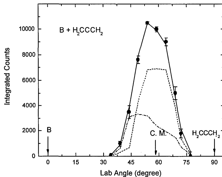
Figure 3: Laboratory angular distribution for the reaction of boron atoms with allene. The corresponding center-of-mass functions contributing to both product isomers are shown in Figure 4.
