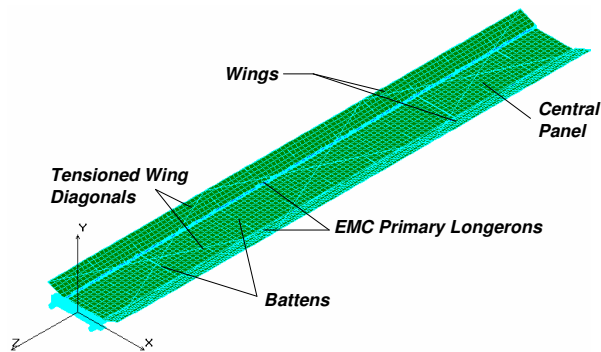
Figure 3. RAPDAR solar array system.
