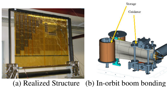
Figure 2. HTS's Flexible Solar Generator 13
