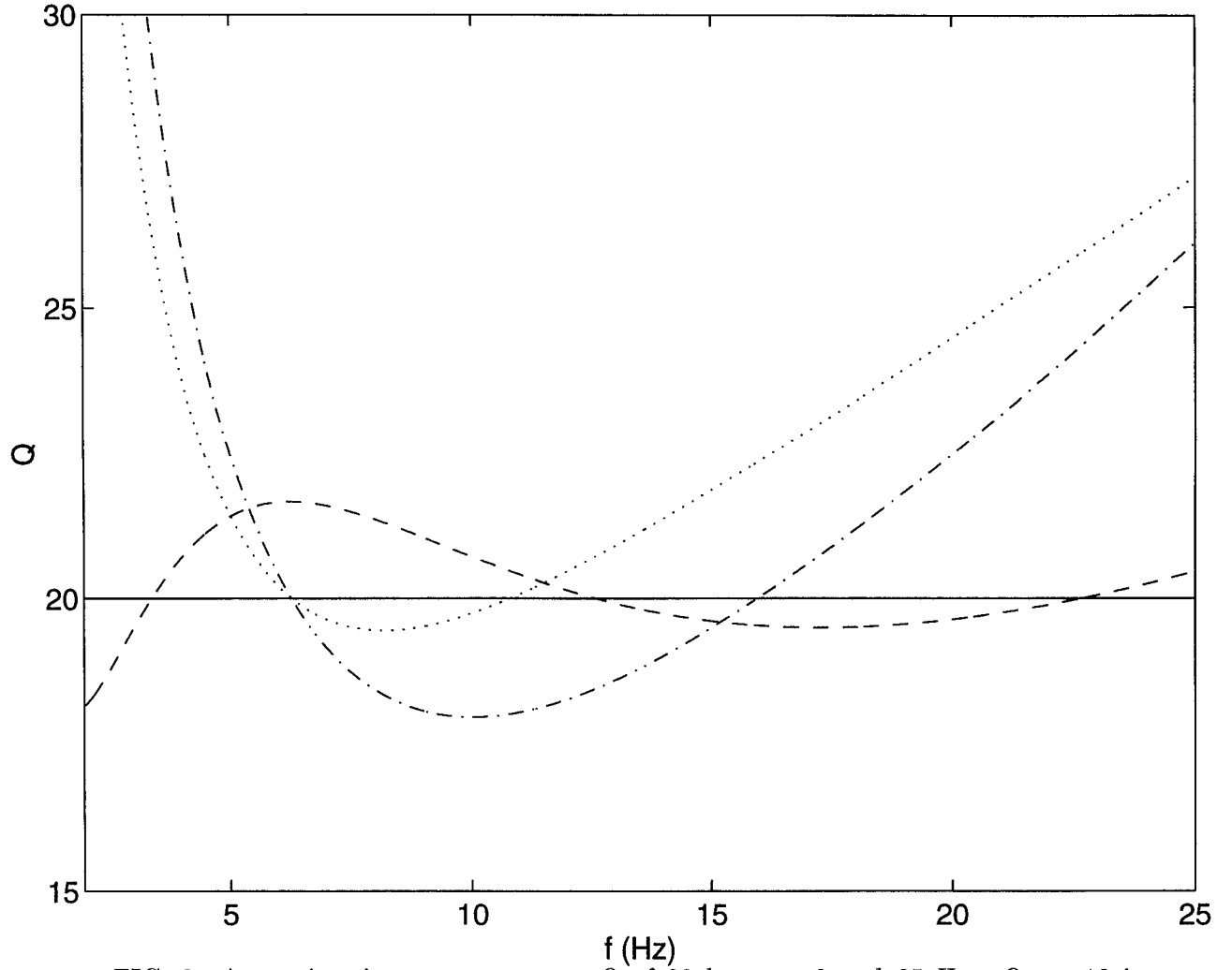
FIG. 2. Approximations to a constant Q of 20 between 2 and 25 Hz. Q_0 \approx 18 in algorithm. Solid: Desired Q . Dashed: \tau -method using two relaxation mechanisms. Dotted: Padé approximant method using two relaxation mechanisms. Dash-dotted: Single relaxation mechanism approximant.
