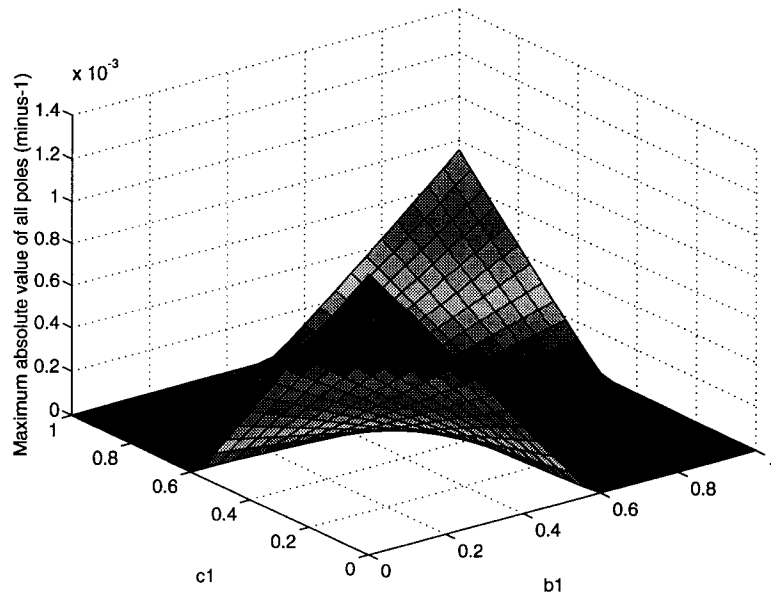
Figure 8: Absolute value of maximum pole for \beta = 1 , a = 0.5 , b_2 = c_2 = 0.5 and varying b_1 and c_1 . Stable schemes occur for (equivalent) staggered stencils and schemes with coefficients approaching the staggered scheme configuration.
