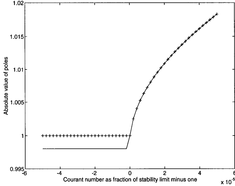
Figure 14: Absolute value of maximum pole and absolute value of pole corresponding to maximum wavenumber. The poles become larger than one exactly at the stability limit in Equation (7). \tau = 0.02 , \eta = 0.2 . Solid - Absolute value of pole corresponding to maximum wavenumber. Plus - The absolute value of the pole with the largest absolute value of all poles for all wavenumbers.
