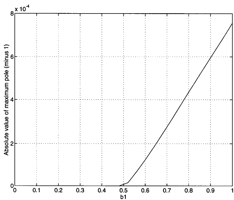
Figure 10: Value of maximum pole minus one. Crank-Nicolson, \beta = 1 . The scheme becomes unstable for b_1 greater than approximately 0.47 < b_1 .
