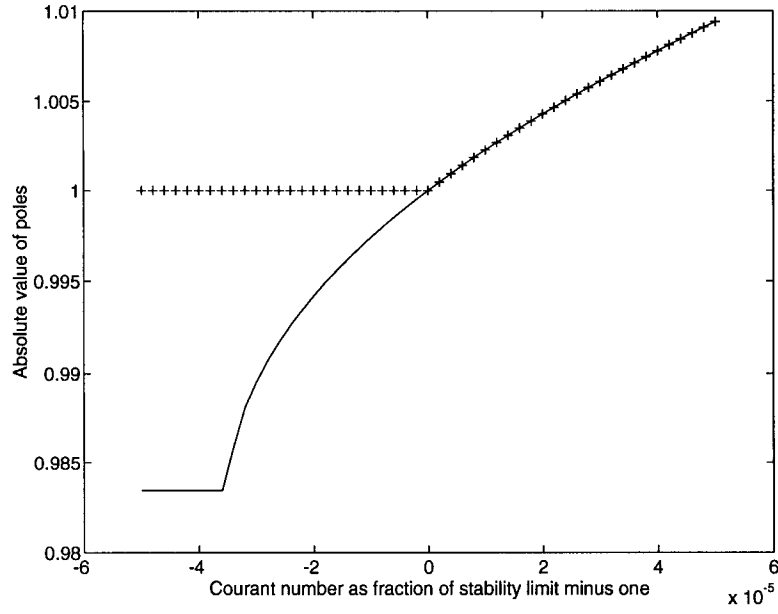
Figure 15: Absolute value of maximum pole and absolute value of pole corresponding to maximum wavenumber. The poles become larger than one exactly at the stability limit in Equation (7). \tau = 0.2 , \eta = 0.2 . Solid - Absolute value of pole corresponding to maximum wavenumber. Plus - The absolute value of the pole with the largest absolute value of all poles for all wavenumbers.
