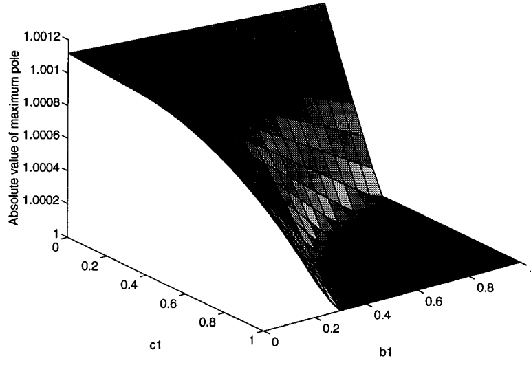
Figure 6: Absolute value of maximum pole for \beta = 0 , a = 0.5 , b_2 = 1 , c_2 = 1 and varying b_1 and c_1 . Stable scheme occurs for large values of c_1 and b_1 .
