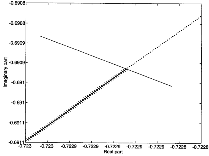
Figure 5: The position of the maximum pole and the pole corresponding to the largest wavenumber. They coincide for small values of c_1 . For large values of c_1 the largest pole corresponds to wavenumber k = 0 and is located at 1 + 0i . Dots and crosses coincide until the scheme is stable. Solid - Part of the unitcircle. Crosses - The position of the largest pole (if inside scale of plot). Dots - Position of pole corresponding to the largest wavenumber.
