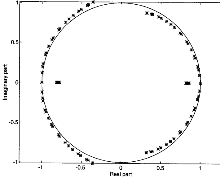
Figure 7: Position of poles for \beta = 1 schemes, for a large value of the attenuation parameter \tau . Clearly unstable. It is always the poles close to -1 , which are outside the unit circle for the unstable schemes.
