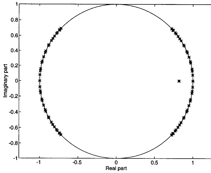
Figure 1: Position of poles for \beta = 0 schemes. Unstable, though not obvious. It is always the poles close to -1 , which are outside the unit circle for the unstable schemes.
