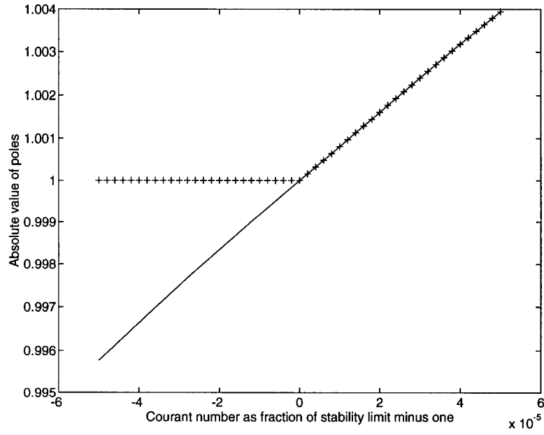
Figure 16: Absolute value of maximum pole and absolute value of pole corresponding to maximum wavenumber. The poles become larger than one exactly at the stability limit in Equation (7). \tau = 0.02 , \eta = 5 . Solid - Absolute value of pole corresponding to maximum wavenumber. Plus - The absolute value of the pole with the largest absolute value of all poles for all wavenumbers.
