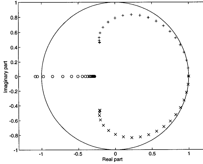
Figure 20: Location of poles (roots) for the Courant number above the stability limit, \eta = 5 and \tau = 0.5 . Two sets of poles closely follow the unit circle for small wavenumbers but have considerably smaller absolute value for large wavenumbers. A purely real pole decreases its value from q , which is its value for 0 wavenumber. The purely real pole passes for some wavenumber the point -1 + 0i and attains an absolute value greater than one. This in contrast to the case \eta = 0.2 where the complex poles became real and their absolute greater than one. The modes corresponding to wavenumbers where the pole is greater than one will numerically explode.
