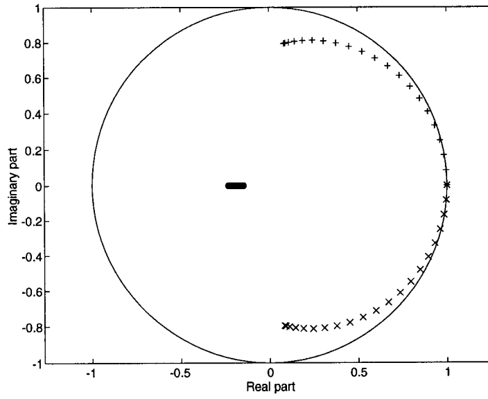
Figure 19: Location of poles (roots) for the Courant number below the stability limit, \eta = 5 and \tau = 0.5 . Two sets of poles closely follow the unit circle for small wavenumbers but have considerably smaller absolute value for large wavenumbers. A purely real pole changes value around q . Here q is negative.
