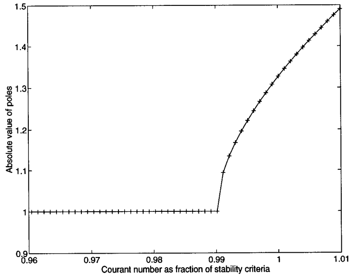
Figure 12: Absolute value of maximum pole and absolute value of pole corresponding to maximum wavenumber. The Courant number is compared to the stability limit in Equation (6). The scheme becomes unstable for a Courant number slightly less than that stability limit. \tau = 0.02 , \eta \rightarrow 0 . Solid - Absolute value of pole corresponding to maximum wavenumber. Plus - The absolute value of the pole with the largest absolute value of all poles for all wavenumbers.
