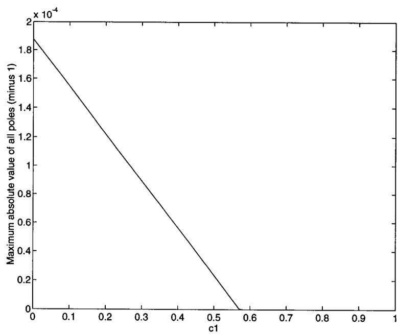
Figure 4: Value of maximum pole minus one. Crank-Nicolson, \beta = 0 . The scheme becomes stable for c_1 greater than approximately 0.55 < c_1 .
