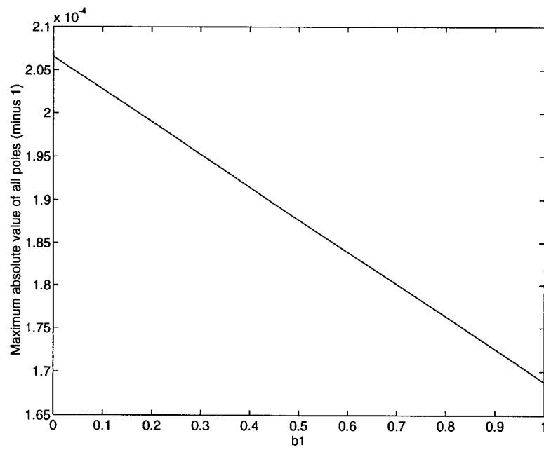
Figure 2: Value of maximum pole minus one. Crank-Nicolson, \beta = 0 . The value is clearly greater than one for all choices of b_1 .
