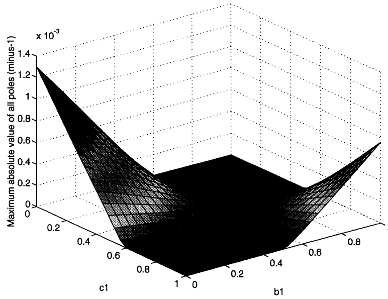
Figure 9: Absolute value of maximum pole for \beta = 1 , a = 0.5 , b_2 = c_2 = 0.5 and varying b_1 and c_1 . Stable schemes occur for (equivalent) staggered stencils and schemes with coefficients approaching the staggered scheme configuration. Other view.
