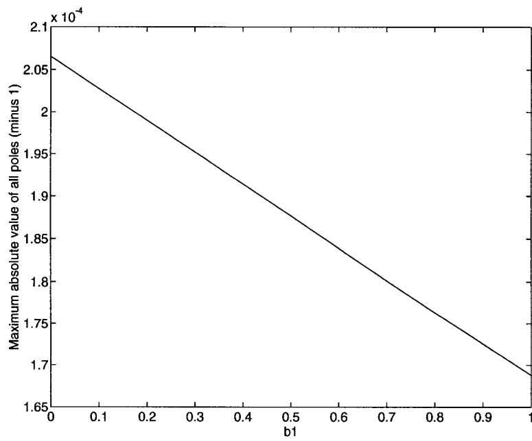
Figure 3: Value of maximum pole minus one. Crank-Nicolson, \beta = 0 . The value is clearly greater than one for all choices of b_1 .
