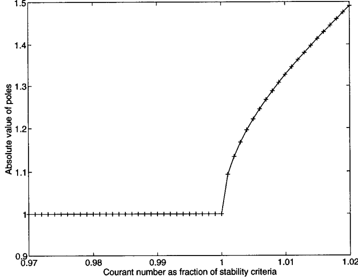
Figure 11: Absolute value of maximum pole and absolute value of pole corresponding to maximum wavenumber. The poles become larger than one exactly at the stability limit. \tau = 0 , \eta \rightarrow 0 . Solid - Absolute value of pole corresponding to maximum wavenumber. Plus - The absolute value of the pole with the largest absolute value of all poles for all wavenumbers.
