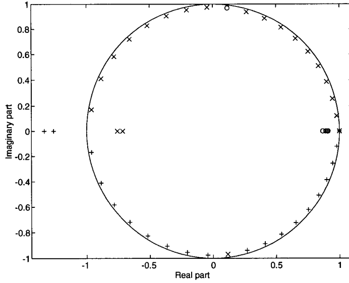
Figure 18: Location of poles (roots) for the Courant number above the stability limit, \eta = 0.2 and \tau = 0.5 . Two sets of poles closely follow the unit circle, whereas a purely real pole changes value around q . The poles following the unit circle pass for some wavenumber the point -1 + 0i and both become purely real. One with an absolute value greater than one and one less than one. The modes corresponding to wavenumbers where the poles are greater than one will numerically explode.
