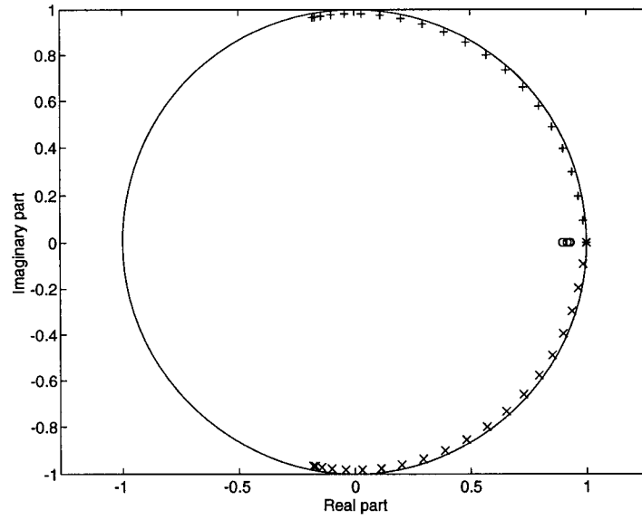
Figure 17: Location of poles (roots) for the Courant number below the stability limit, \eta = 0.2 and \tau = 0.5 . Two sets of poles closely follow the unit circle, whereas a purely real pole changes value around q .
