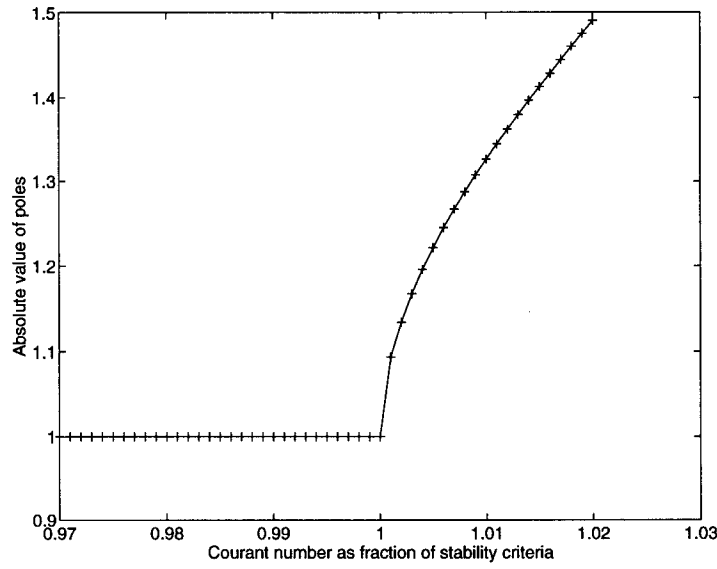
Figure 13: Absolute value of maximum pole and absolute value of pole corresponding to maximum wavenumber. The poles become larger than one exactly at the stability limit in Equation (7). \tau = 0.02 , \eta \rightarrow 0 . Solid - Absolute value of pole corresponding to maximum wavenumber. Plus - The absolute value of the pole with the largest absolute value of all poles for all wavenumbers.
