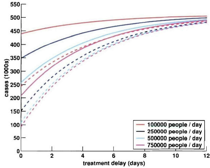
Figure 12. The number of symptomatic people as a function of delay in initiating a public health response, assuming a prophylaxis efficacy of 90%. This figure shows four possible distribution rates for prophylaxis. Solid lines correspond to the assumption that the metropolitan region will seek prophylaxis, while the dashed lines correspond to only those in the plume plus an extra 50,000 people demanding prophylaxis.
