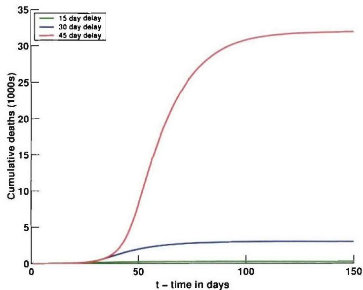
Figure 6. The cumulative number of deaths resulting from the contemporary outbreak, D(t) .
