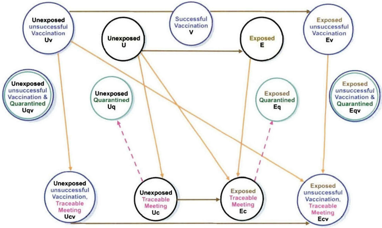
Figure 3. A schematic of the transitions allowed when contact tracing is followed by quarantine. The color coding of the arrows and circles is the same as that in Figure 2; pink arrows indicate transitions due to contact tracing and quarantining if there is capacity.
