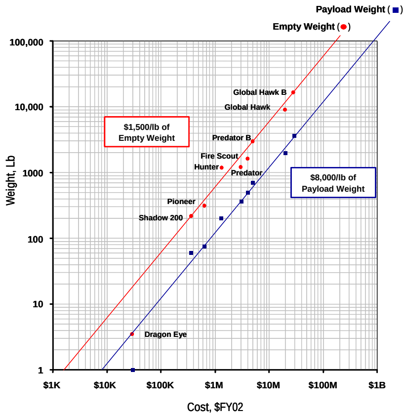
FIGURE 4.3-3. UA CAPABILITY METRIC: WEIGHT V. COST.
