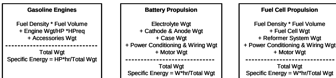
FIGURE D-4. SPECIFIC ENERGY CALCULATION.
