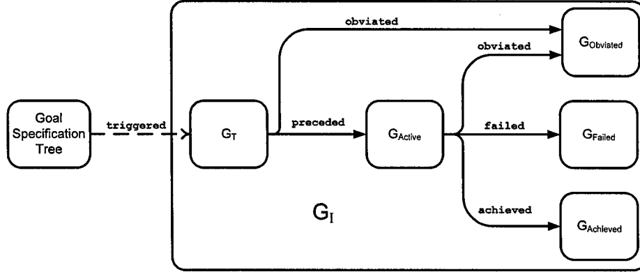
Figure 15. Goal Lifecycle
