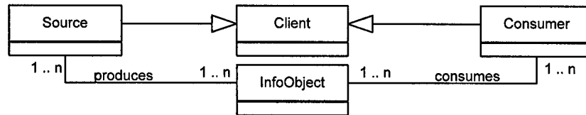
Figure 19. Domain Model
