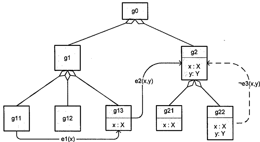
Figure 4. Goal Specification Tree
