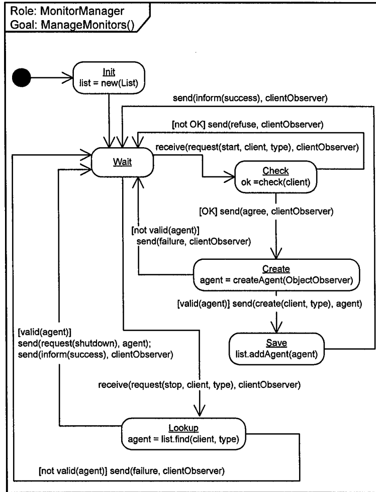
Figure 22. Agent Plan Model for AgentManager
