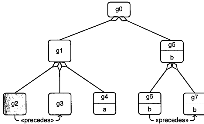
Figure 10. Goal Instance Tree after event e2(b)
