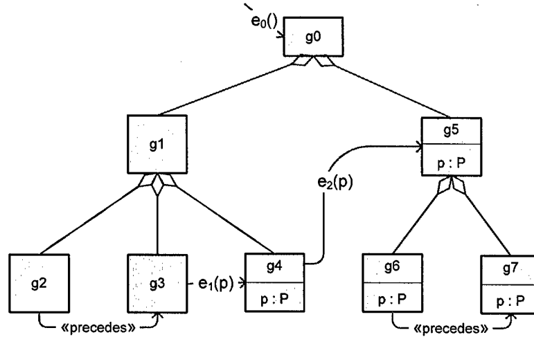
Figure 5. Example Goal Specification Tree
