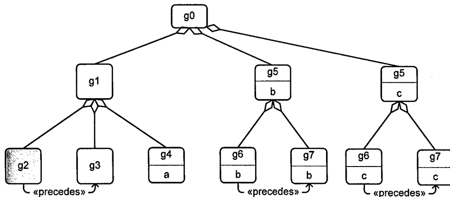
Figure 11. Goal Instance Tree after Event e2(c)
