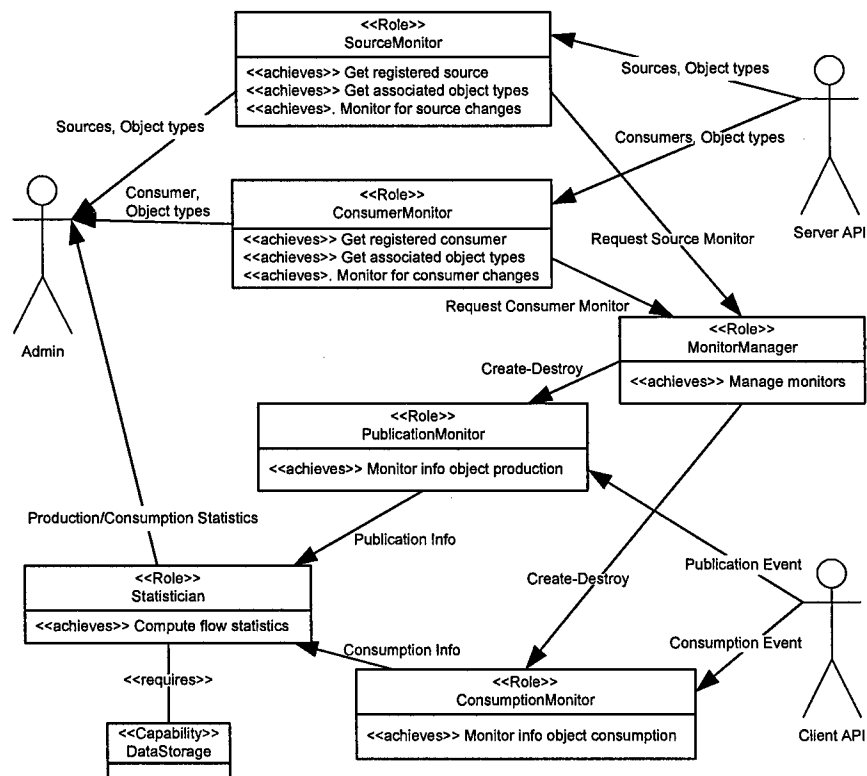
Figure 18. Role Model
