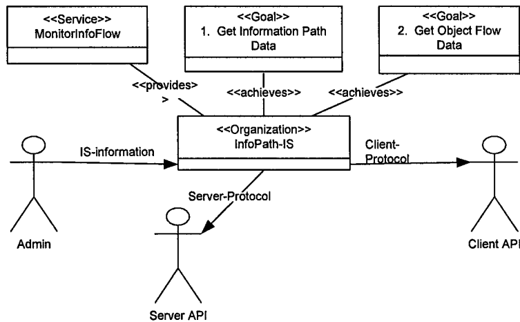
Figure 17. Organization Model
