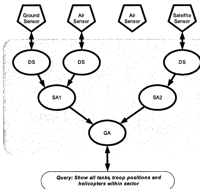
Figure 1. Original System Organization
