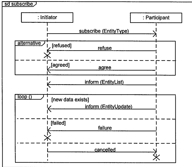
Figure 21. Protocol Model
