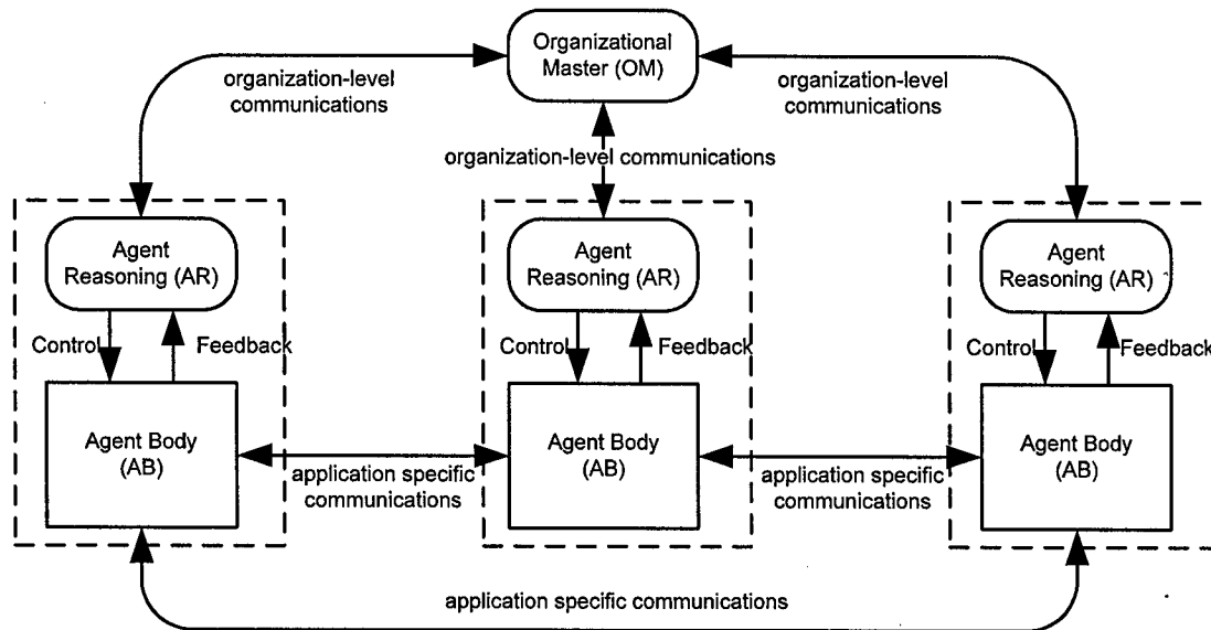
Figure 25. Centralized Architecture
