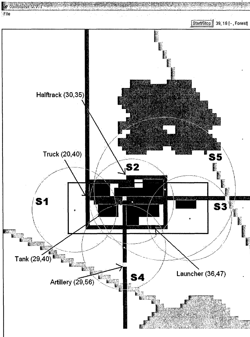
Figure 26. Battlefield Map
