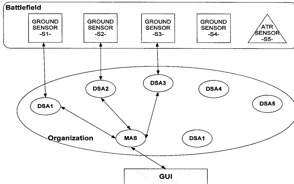
Figure 28. Normal Execution
