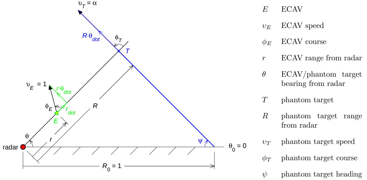
Figure 2. Variables and relations for a constant-speed ECAV and a constant-speed constant-course phantom track.
