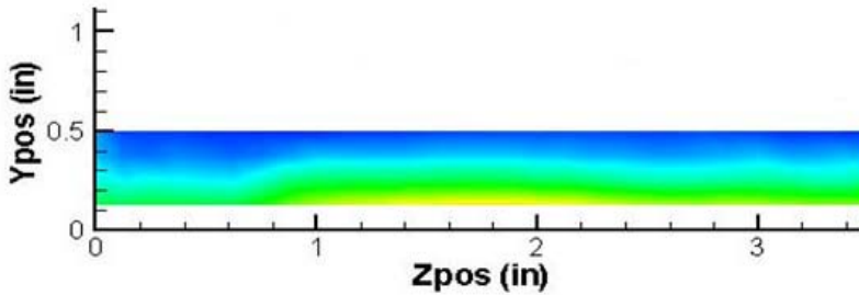
Figure 33. Enthalpy distributions behind cavity ramp with flow out of page. Fuel injection rate is 32% and air injection rates are 0, 30, and 70%. Fuel and air percentages are to the right (F_X A_Y, X = %ethylene Y = %air). The color shading scheme is the same for all pictures.
