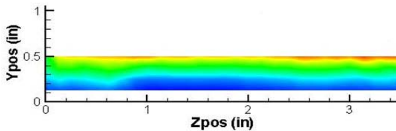
Figure 37. Total pressure distributions behind cavity ramp with flow out of page. Fuel injection rate is 32% and air injection rates are 0, 30, and 70%. Fuel and air percentages are to the right (F_X A_Y, X = %ethylene Y = %air). The color shading scheme is the same for all pictures.
