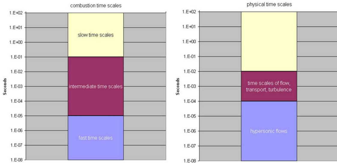
Figure 3. Range of physical and chemical timescales for hydrocarbon combustion (reproduced without permission from Maurice et al., 2000).
