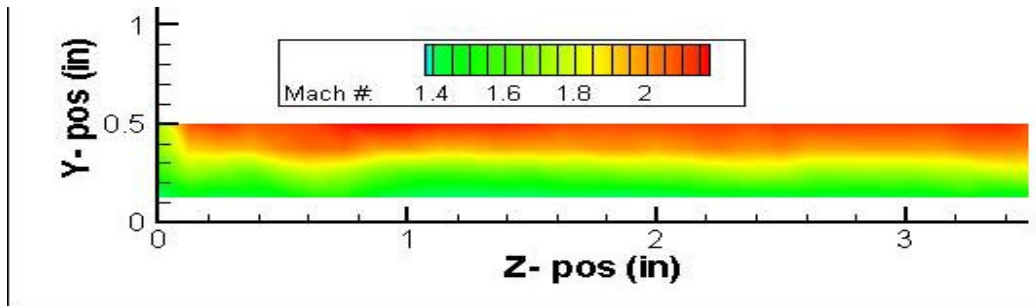
Figure 20. Mach number distribution behind cavity ramp for non-reacting flow (flow out of page).
