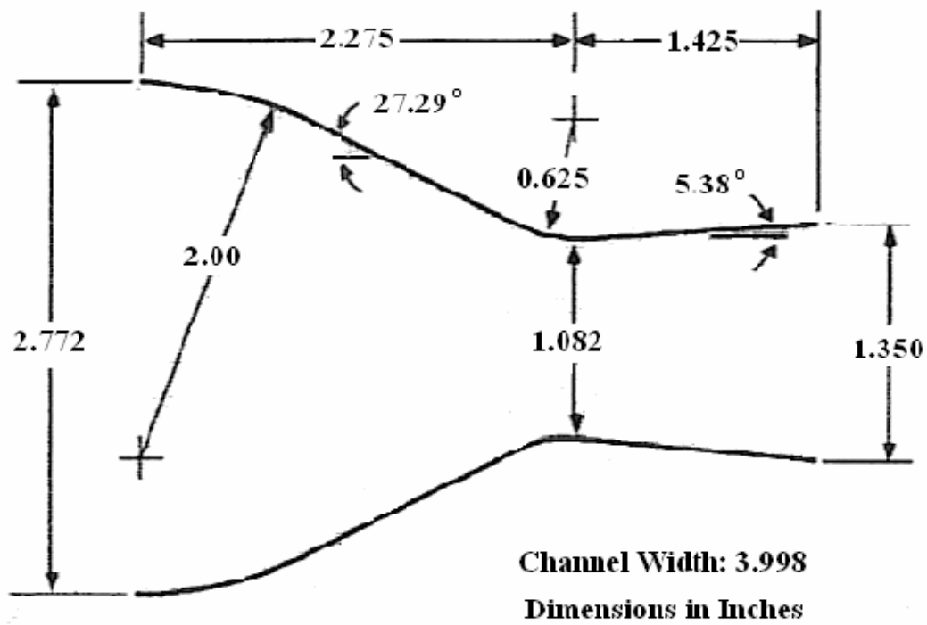
Figure A8: Nozzle geometry [20].
