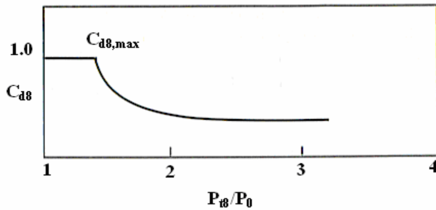
Figure 2.2 Nozzle discharge coefficient versus pressure ratio for a C-D nozzle [2].
