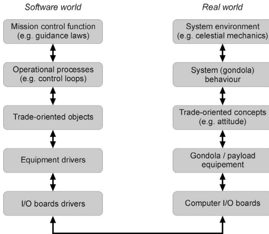
Figure 3-3 : Layer-oriented view of software architecture
