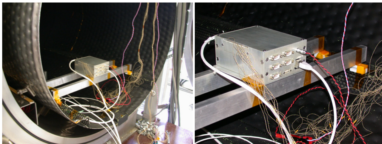
Figure 4-1 : Operational IP router after vacuum & thermal environment tests
