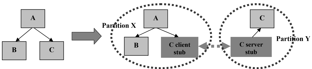
Figure 3-2 : GLADE's process for partition generation
