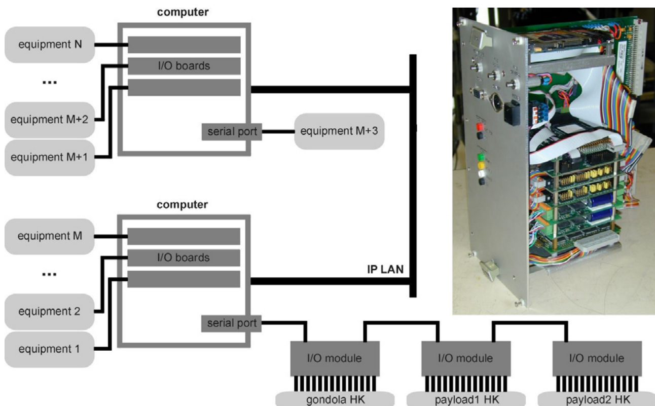
Figure 2-3 : A typical on-board computer architecture (left) and a PC104 stack (right)
