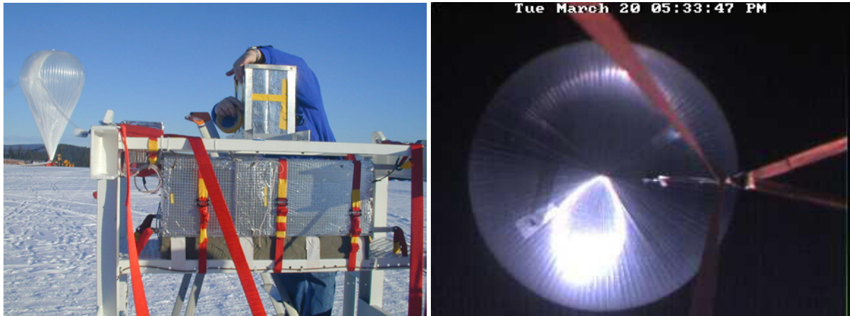
Figure 3-6 : First flight of IP router prototype – test gondola a few minutes before launch (left), balloon at float, seen with an on-board webcam (right)
