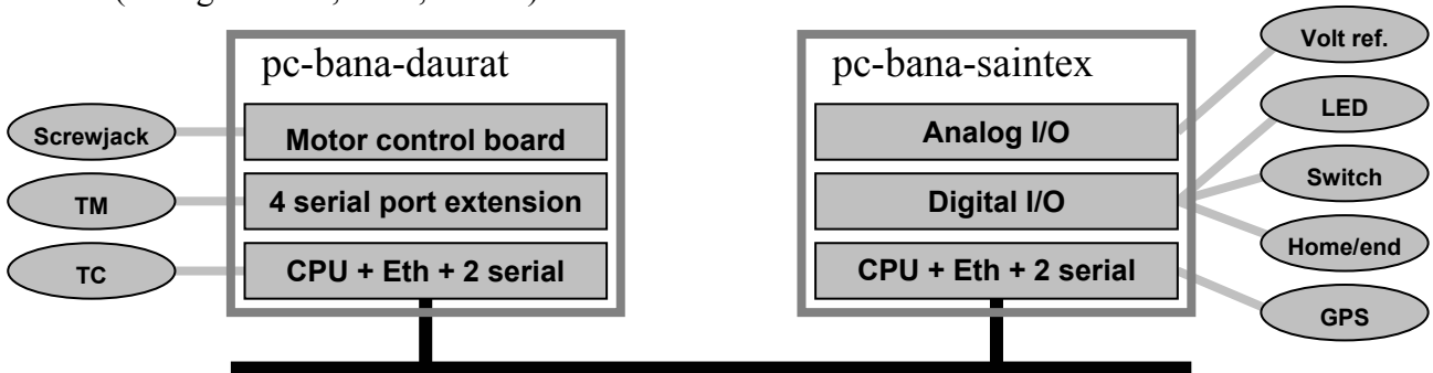
Figure 3-4 : Distributed mock-up hardware configuration
