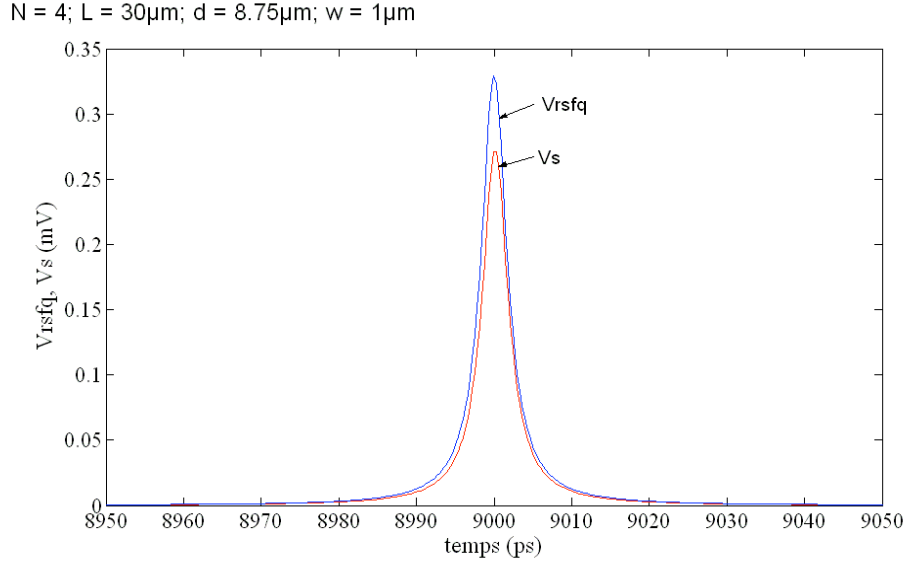
Figure 9 - Input (blue curve) and output (red curve) signal associated to the photoswitch under study in the ON mode. One can notice that RSFQ signal is correctly transmitted through the photoswitch.
