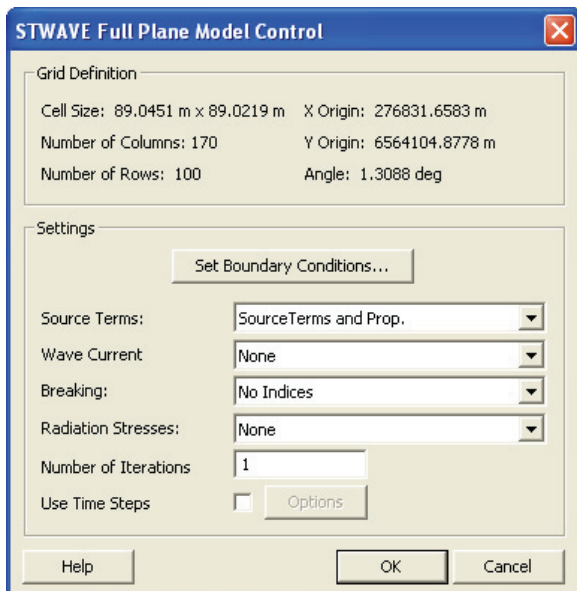
Figure 7. STWAVE-FP Model Control dialog
