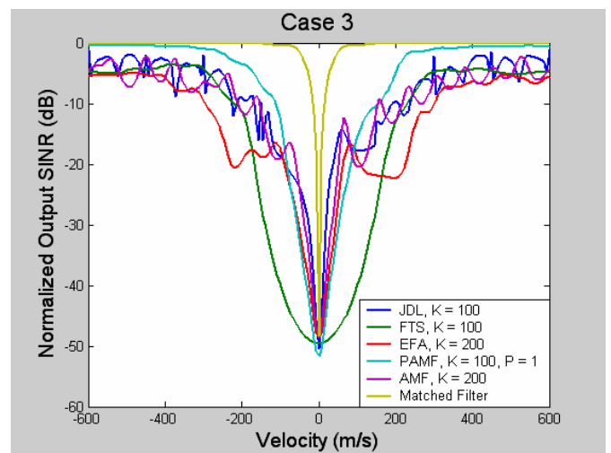
Figure 12 Normalized Output SINR vs. Target Velocity
