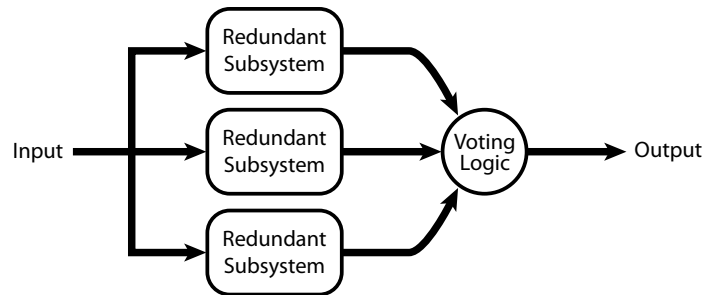
Figure 2: Modular Redundancy
