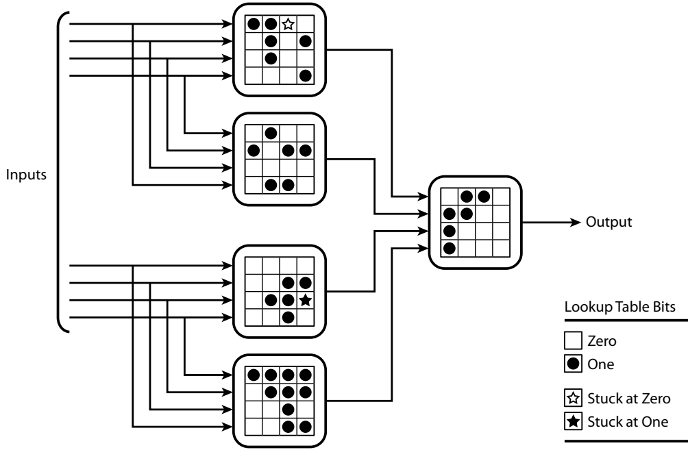
Figure 6: Example Test Circuit Model
