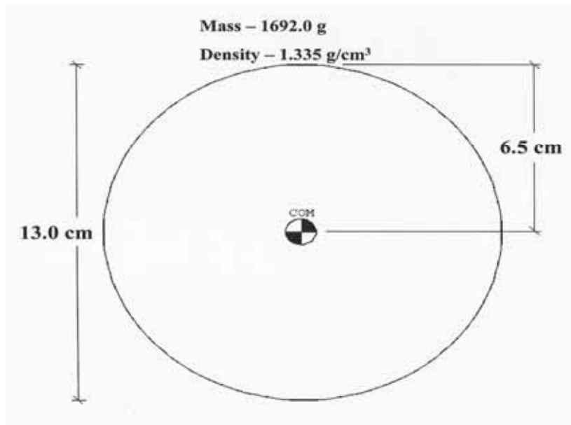
Figure 7. Diagram of Sphere Shaped Model Mine.
