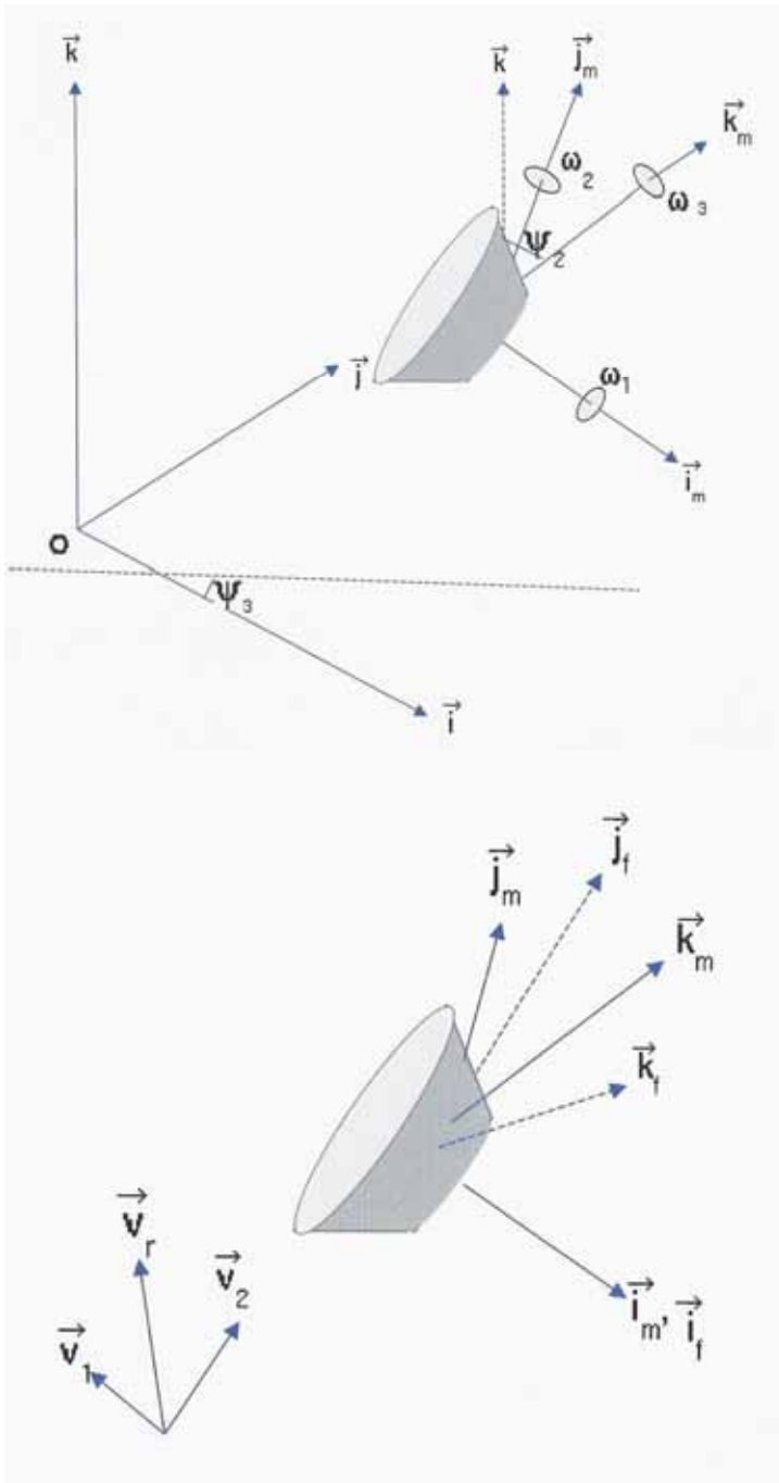
Figure 5. Three coordinate systems for Manta shape.
