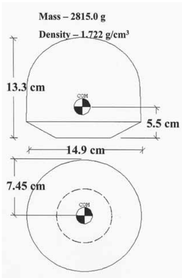
Figure 9. Diagram of Gumdrop Shaped Model Mine.
