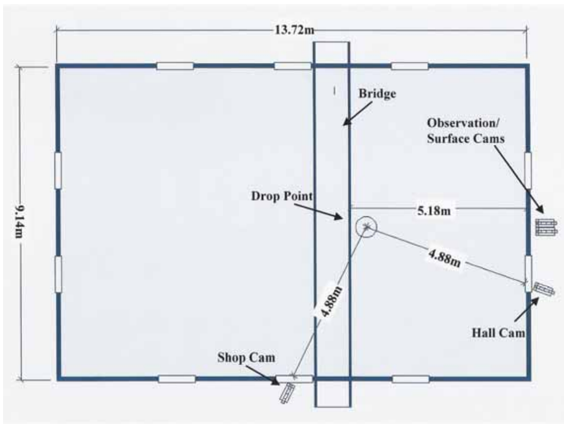
Figure 17. MIDEX II Tank Set Up Top View.
