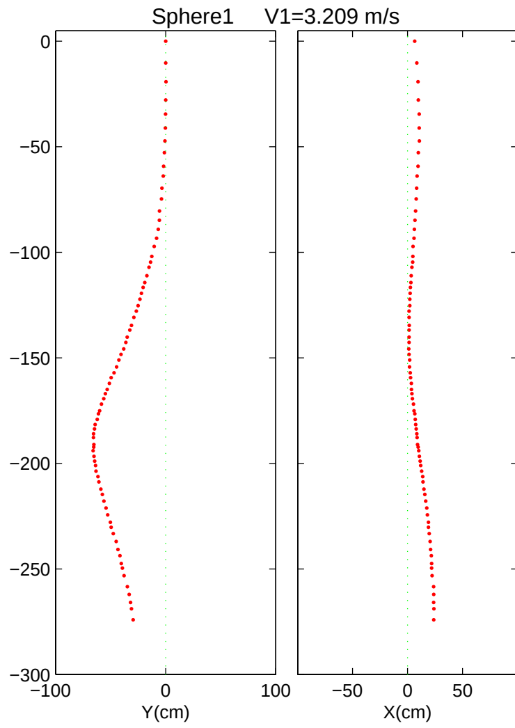
Figure 23. Sample X-Z/Y-Z Trajectory Plot.
