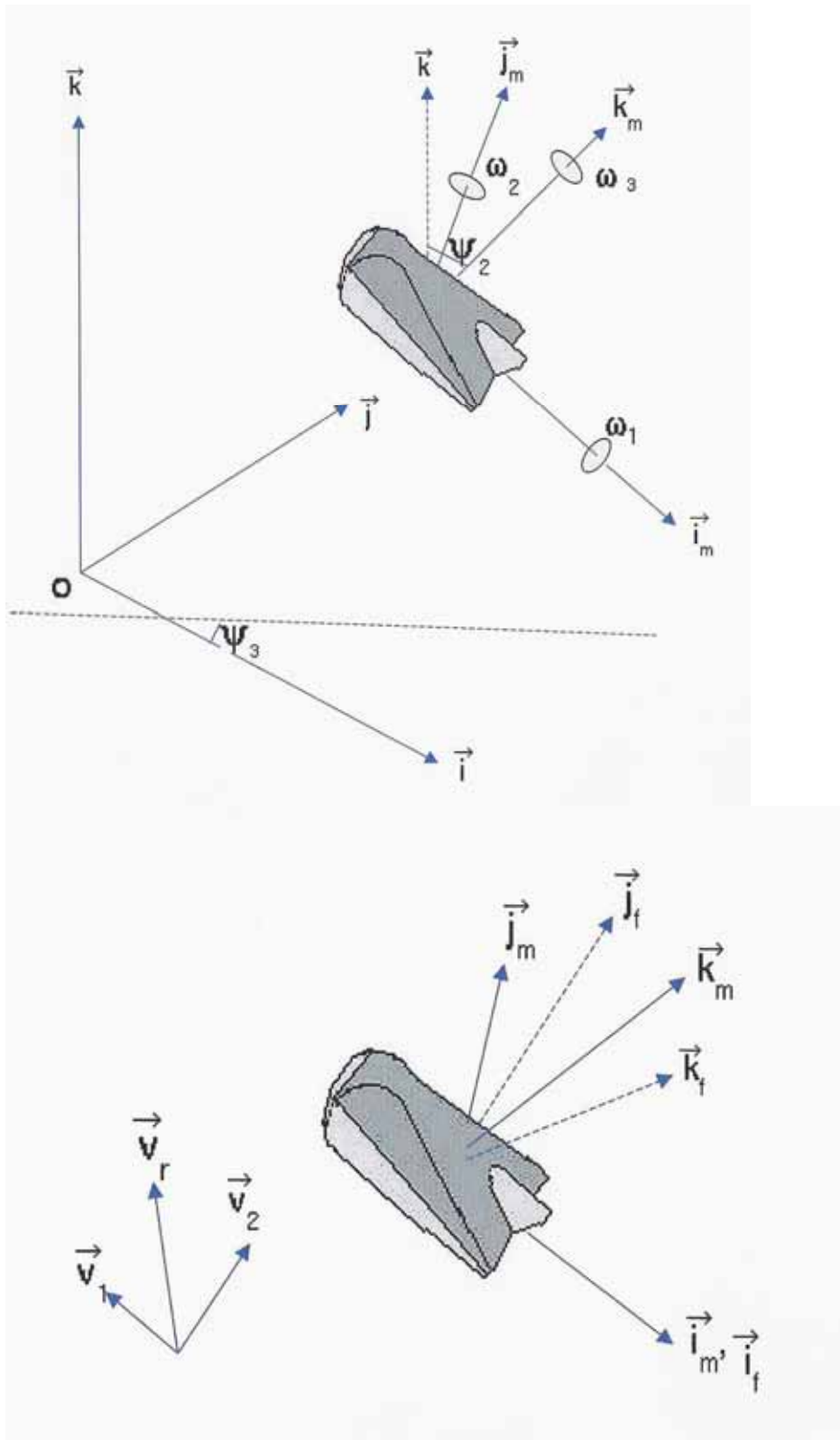
Figure 6. Three coordinate systems for Rockan shape.
