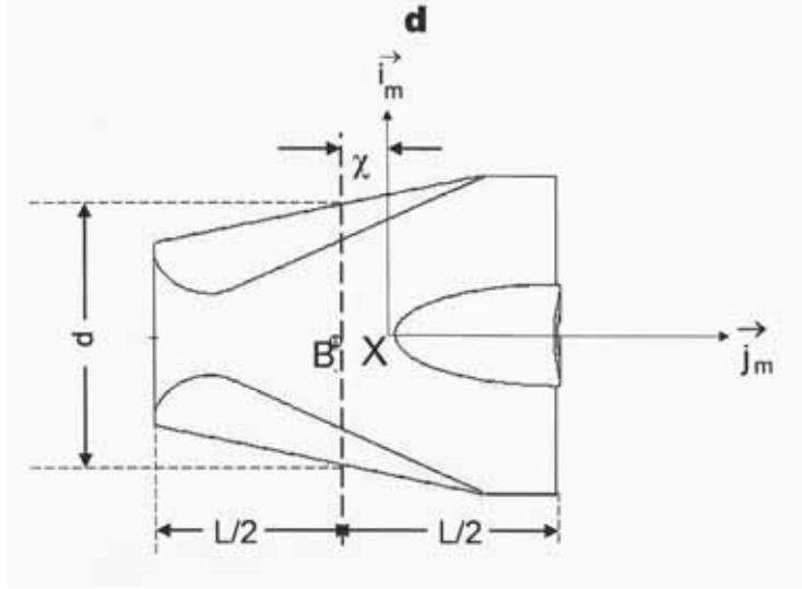
Figure 4b. M-coordinate with the COM as the origin \mathbf{X} and (\mathbf{i}_m, \mathbf{j}_m) as the two axes. Here, \chi is the distance between the COV (B) and COM, (L, d) are the shape's length and diameter.
