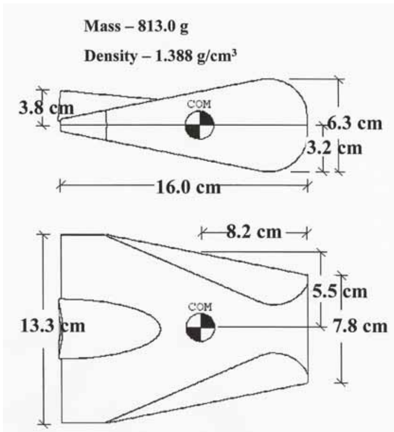
Figure 13. Diagram of Rockan Shaped Model Mine.
