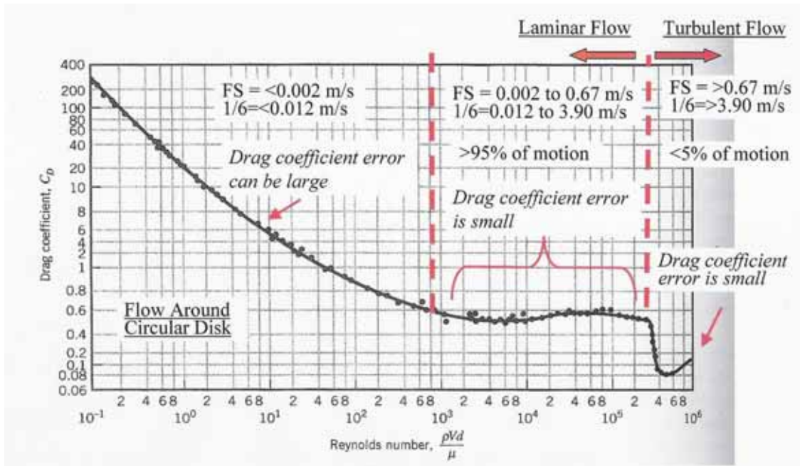
Figure 30. Drag Coefficient vs. Reynolds Number for Flow Around a Circular Disk (After Gefken, 2005).
