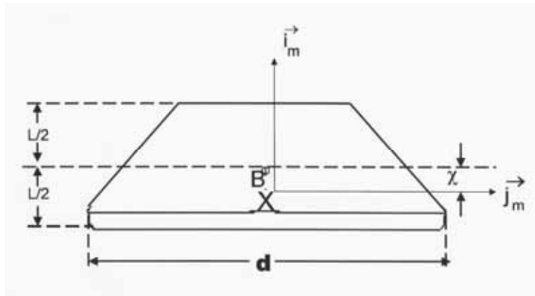
Figure 4a. M-coordinate with the COM as the origin \mathbf{X} and (\mathbf{i}_m, \mathbf{j}_m) as the two axes. Here, \chi is the distance between the COV ( \mathbf{B} ) and COM, (L, d) are the shape's length and diameter.
