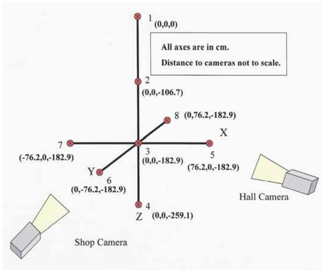
Figure 20. Diagram of Calibration Test Cross.
