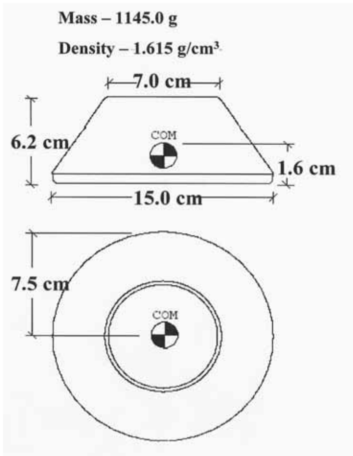
Figure 11. Diagram of Manta Shaped Model Mine.
