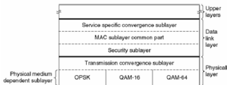
Figure 14. 802.16 Data Link Layer 32
